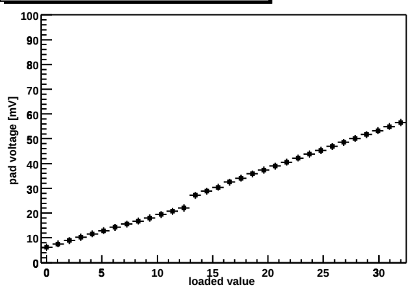
Chip Z36459A-W03-X11-Y14 shaper DAC
