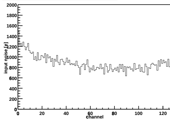
Chip Z36459A-W03-X11-Y14 Input noise vs. channel
