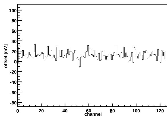
Chip Z36459A-W03-X11-Y14 Offset vs. channel
