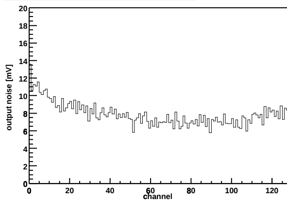
Chip Z36459A-W03-X11-Y14 Output noise vs. channel
