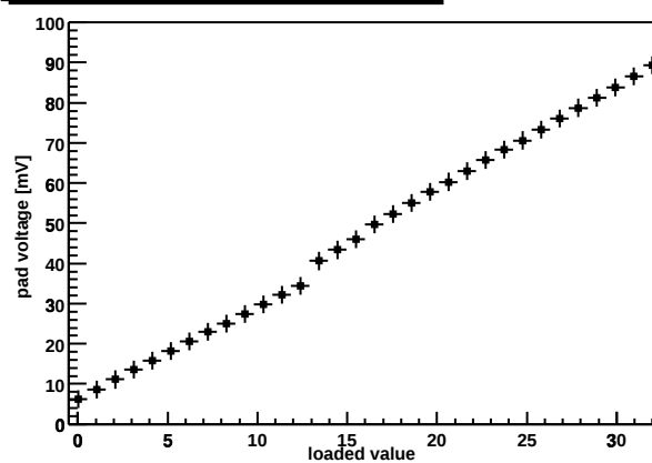
Chip Z36459A-W03-X11-Y14 preamp DAC
