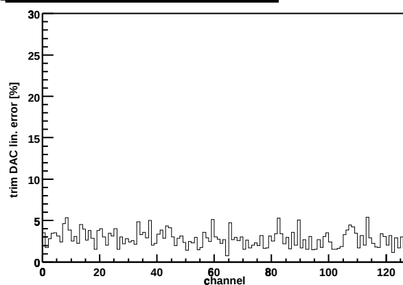
Chip Z36459A-W03-X11-Y14 trim DAC lin. error
