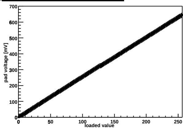
Chip Z36459A-W03-X11-Y14 threshold DAC
