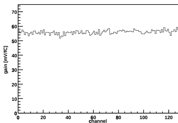
Chip Z36459A-W03-X11-Y14 Gain vs. channel
