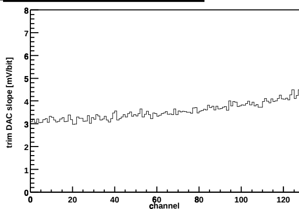
Chip Z36459A-W03-X11-Y14 Trim DAC slope vs. channel
