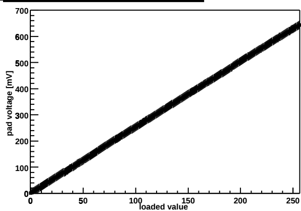
Chip Z36459A-W03-X12-Y03 threshold DAC
