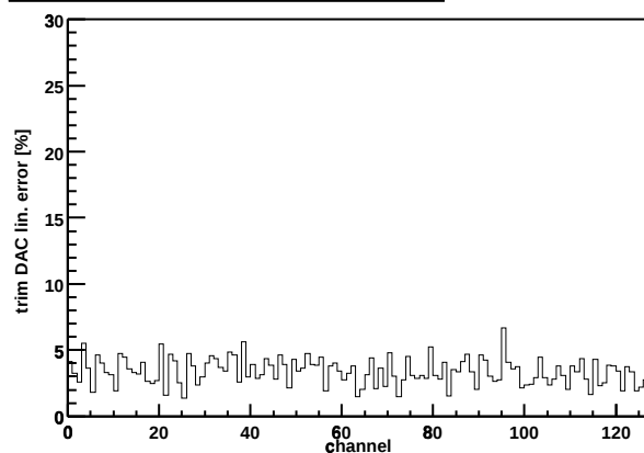
Chip Z36459A-W03-X12-Y03 trim DAC lin. error
