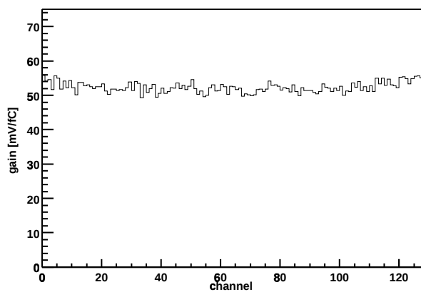
Chip Z36459A-W03-X12-Y03 Gain vs. channel
