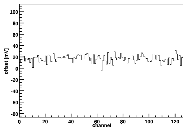
Chip Z36459A-W03-X12-Y03 Offset vs. channel
