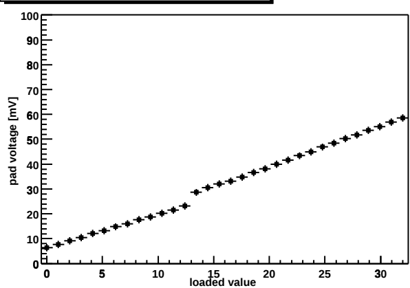
Chip Z36459A-W03-X12-Y03 shaper DAC
