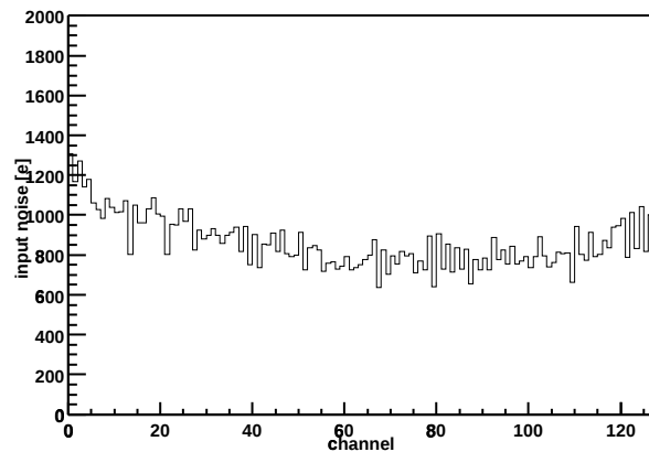
Chip Z36459A-W03-X12-Y03 Input noise vs. channel
