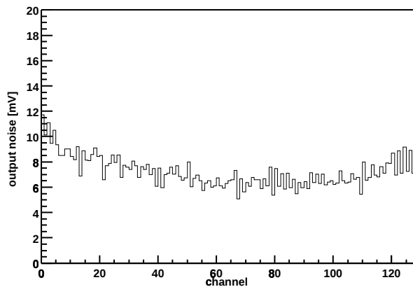
Chip Z36459A-W03-X12-Y03 Output noise vs. channel
