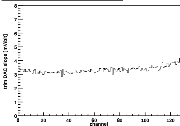
Chip Z36459A-W03-X12-Y03 Trim DAC slope vs. channel
