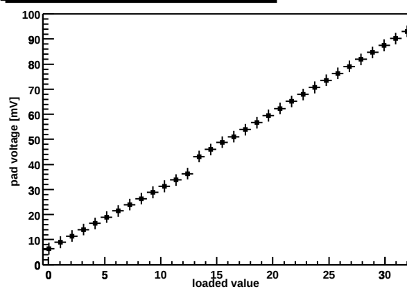
Chip Z36459A-W03-X12-Y03 preamp DAC
