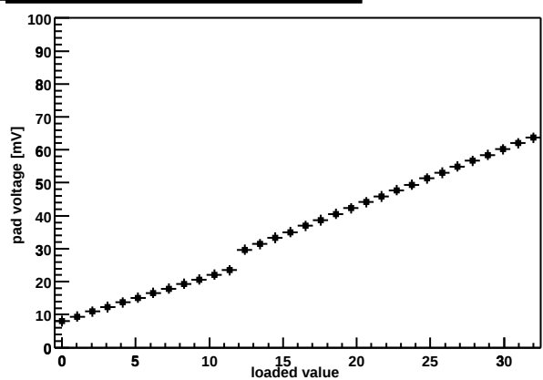
Chip Z36459A-W03-X12-Y11 shaper DAC
