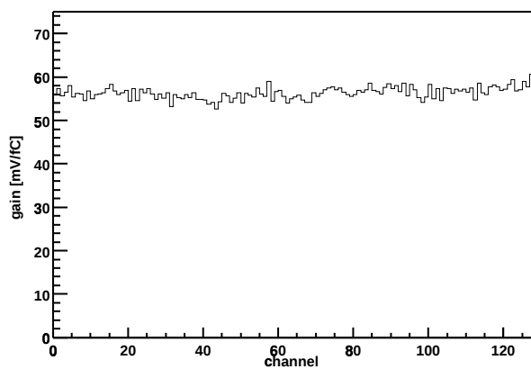
Chip Z36459A-W03-X12-Y11 Gain vs. channel
