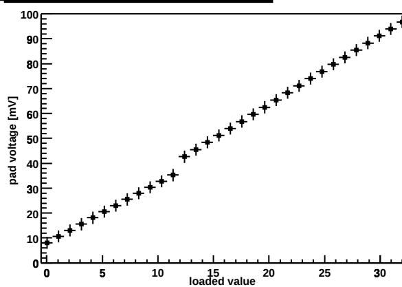
Chip Z36459A-W03-X12-Y11 preamp DAC
