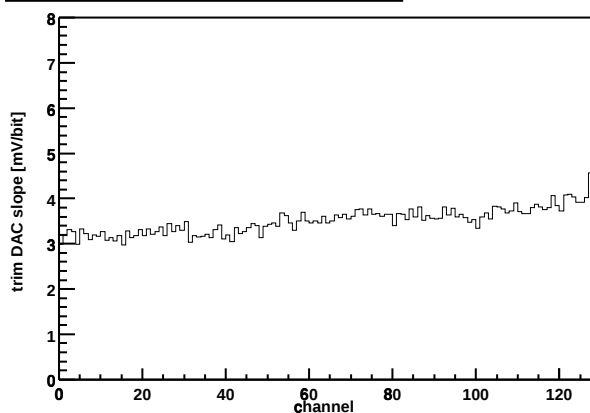
Chip Z36459A-W03-X12-Y11 Trim DAC slope vs. channel
