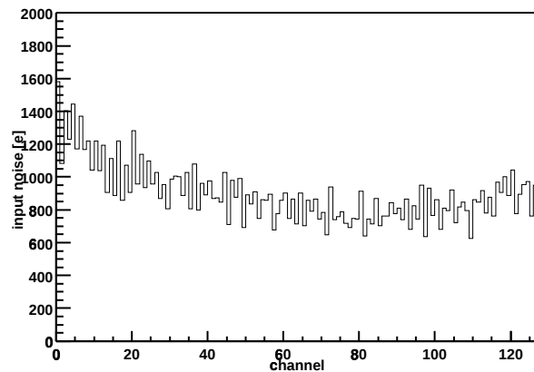
Chip Z36459A-W03-X12-Y11 Input noise vs. channel
