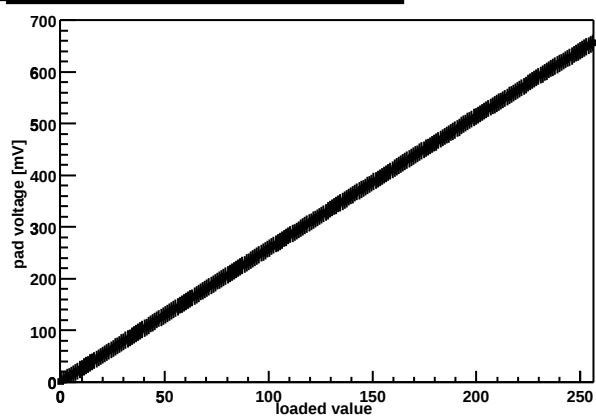
Chip Z36459A-W03-X12-Y11 threshold DAC
