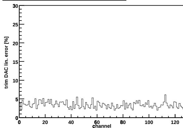
Chip Z36459A-W03-X12-Y11 trim DAC lin. error
