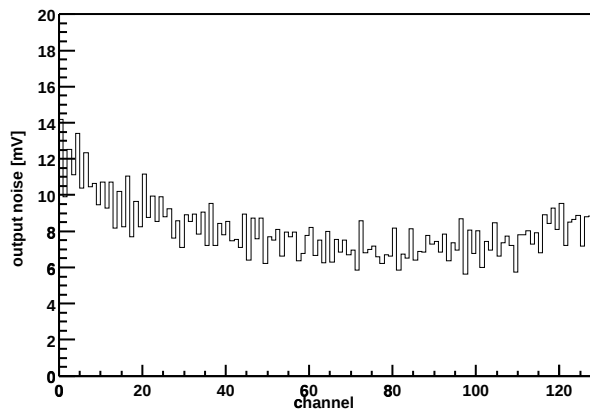
Chip Z36459A-W03-X12-Y11 Output noise vs. channel
