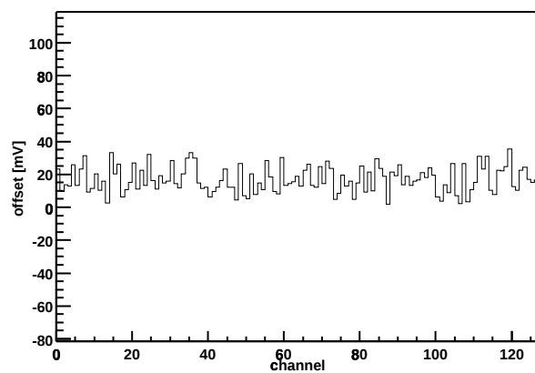
Chip Z36459A-W03-X12-Y11 Offset vs. channel
