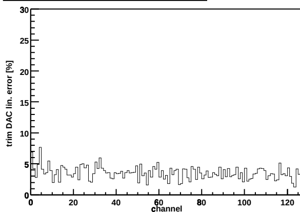
Chip Z36459A-W03-X12-Y12 trim DAC lin. error
