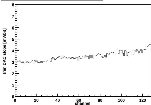
Chip Z36459A-W03-X12-Y12 Trim DAC slope vs. channel
