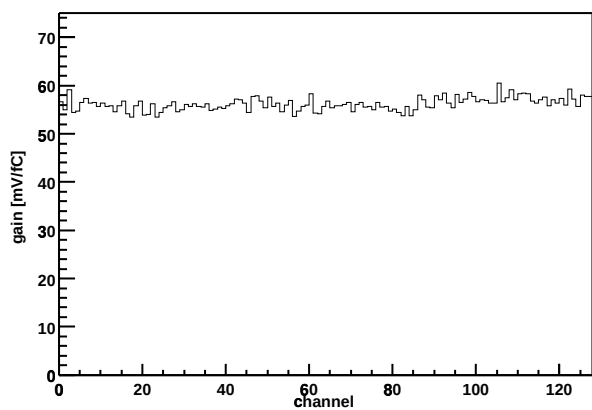
Chip Z36459A-W03-X12-Y12 Gain vs. channel
