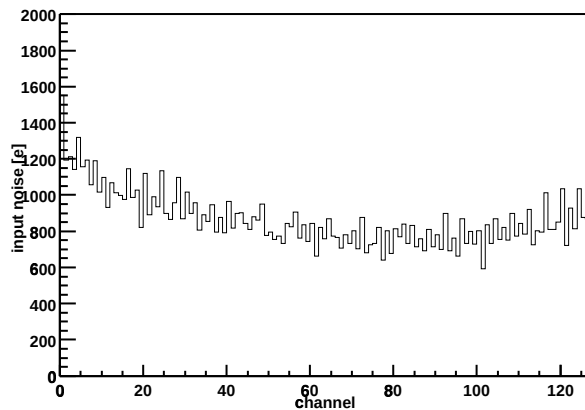
Chip Z36459A-W03-X12-Y12 Input noise vs. channel
