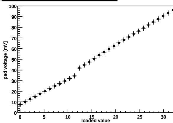
Chip Z36459A-W03-X12-Y12 preamp DAC
