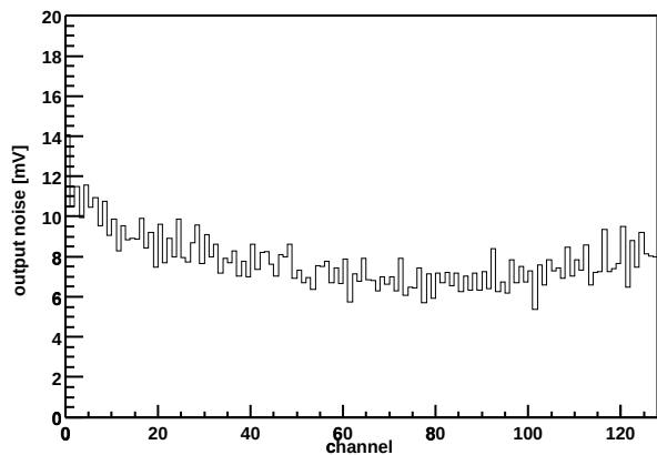
Chip Z36459A-W03-X12-Y12 Output noise vs. channel
