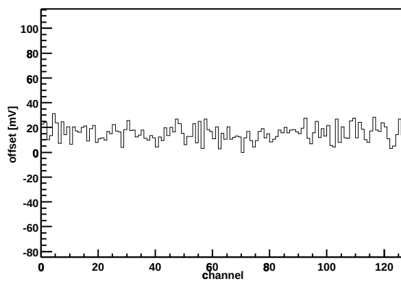
Chip Z36459A-W03-X12-Y12 Offset vs. channel
