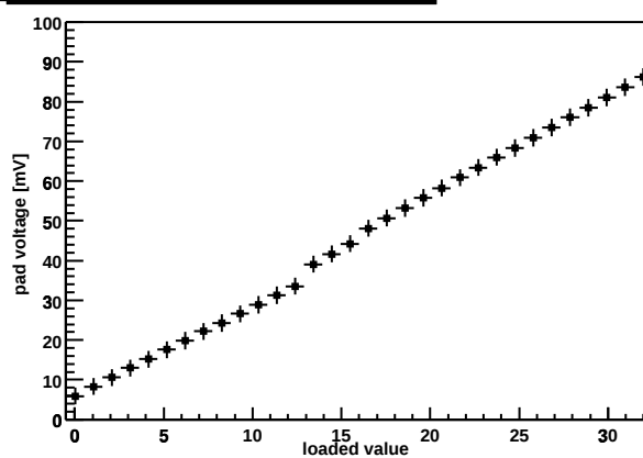
Chip Z36459A-W03-X12-Y15 preamp DAC
