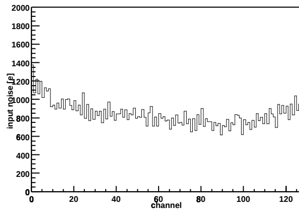
Chip Z36459A-W03-X12-Y15 Input noise vs. channel
