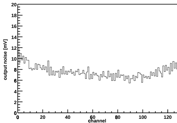
Chip Z36459A-W03-X12-Y15 Output noise vs. channel
