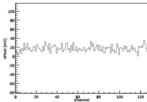
Chip Z36459A-W03-X12-Y15 Offset vs. channel
