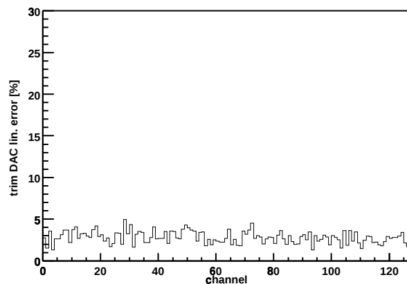
Chip Z36459A-W03-X12-Y15 trim DAC lin. error
