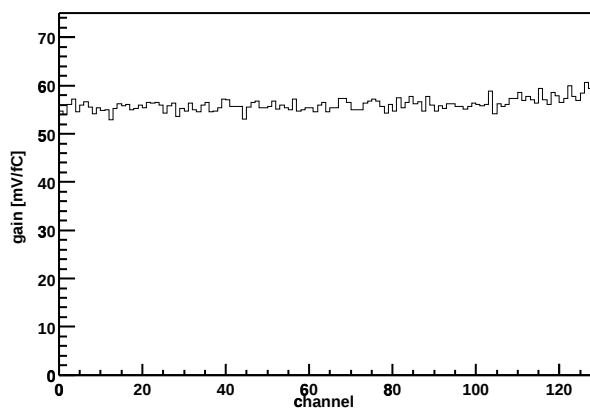
Chip Z36459A-W03-X12-Y15 Gain vs. channel
