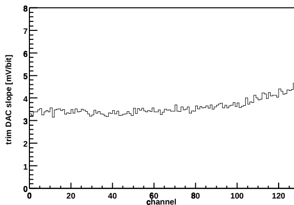
Chip Z36459A-W03-X12-Y15 Trim DAC slope vs. channel
