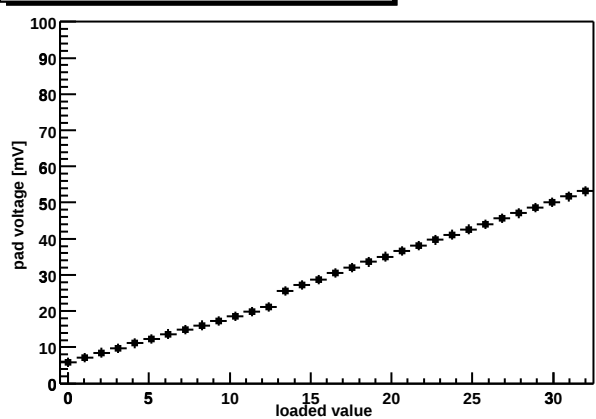
Chip Z36459A-W03-X12-Y15 shaper DAC
