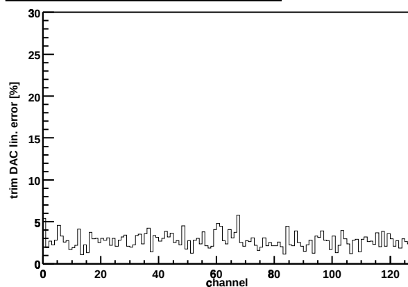
Chip Z36459A-W03-X12-Y16 trim DAC lin. error
