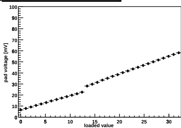
Chip Z36459A-W03-X12-Y16 shaper DAC
