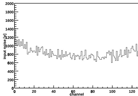
Chip Z36459A-W03-X12-Y16 Input noise vs. channel
