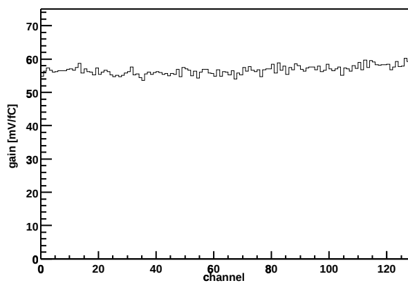
Chip Z36459A-W03-X12-Y16 Gain vs. channel
