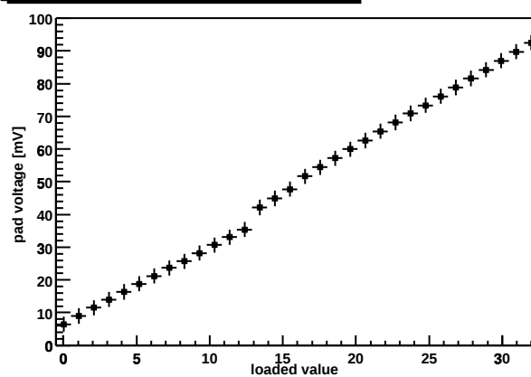
Chip Z36459A-W03-X12-Y16 preamp DAC
