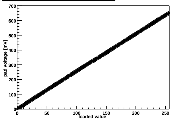
Chip Z36459A-W03-X12-Y16 threshold DAC
