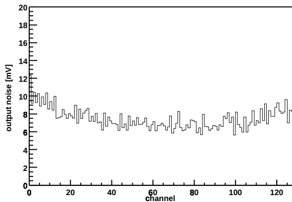
Chip Z36459A-W03-X12-Y16 Output noise vs. channel
