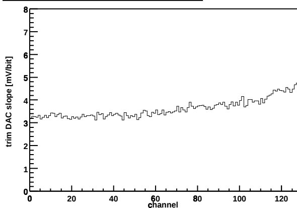
Chip Z36459A-W03-X12-Y16 Trim DAC slope vs. channel
