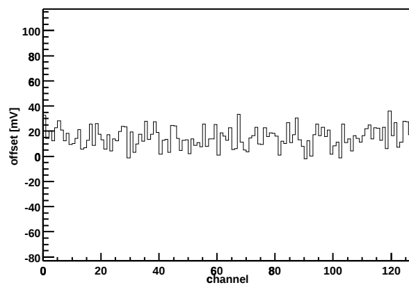
Chip Z36459A-W03-X12-Y16 Offset vs. channel
