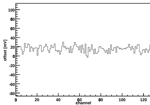
Chip Z36459A-W03-X13-Y15 Offset vs. channel
