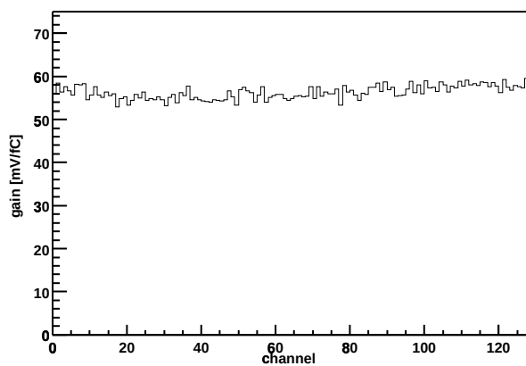
Chip Z36459A-W03-X13-Y15 Gain vs. channel
