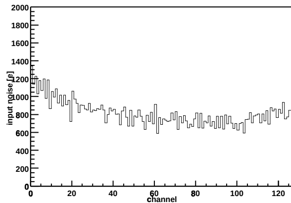
Chip Z36459A-W03-X13-Y15 Input noise vs. channel
