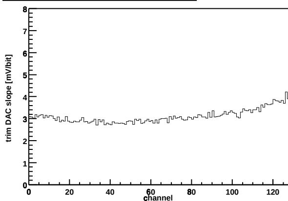
Chip Z36459A-W03-X13-Y15 Trim DAC slope vs. channel
