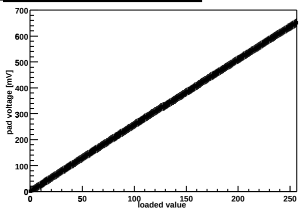
Chip Z36459A-W03-X13-Y15 threshold DAC
