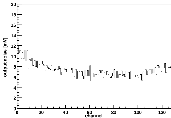
Chip Z36459A-W03-X13-Y15 Output noise vs. channel
