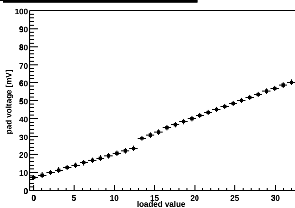
Chip Z36459A-W03-X13-Y15 shaper DAC
