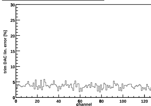
Chip Z36459A-W03-X13-Y15 trim DAC lin. error
