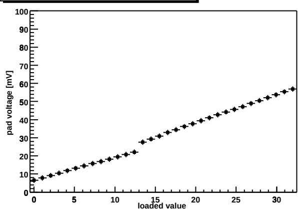
Chip Z36459A-W03-X13-Y16 shaper DAC
