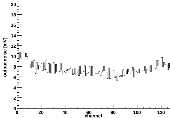
Chip Z36459A-W03-X13-Y16 Output noise vs. channel
