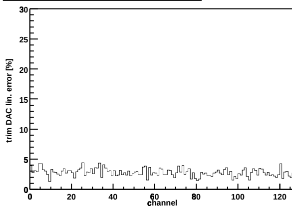
Chip Z36459A-W03-X13-Y16 trim DAC lin. error
