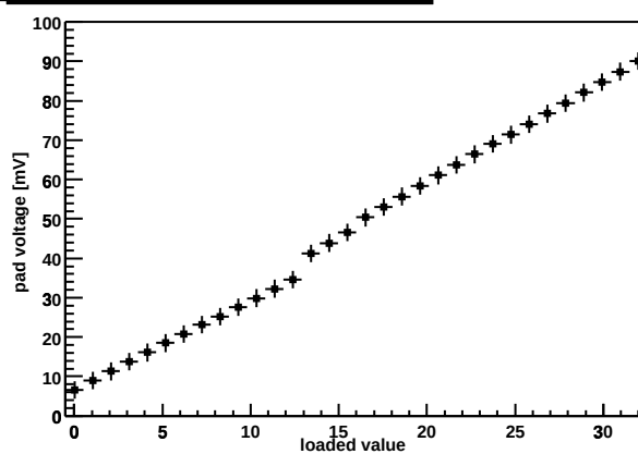
Chip Z36459A-W03-X13-Y16 preamp DAC
