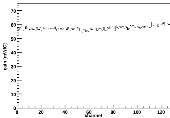
Chip Z36459A-W03-X13-Y16 Gain vs. channel
