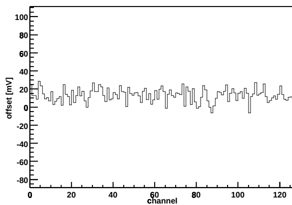
Chip Z36459A-W03-X13-Y16 Offset vs. channel
