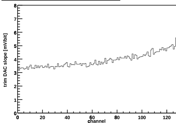
Chip Z36459A-W03-X13-Y16 Trim DAC slope vs. channel
