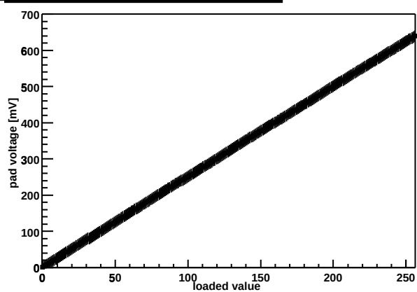
Chip Z36459A-W03-X13-Y16 threshold DAC
