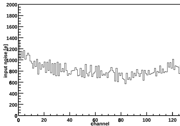
Chip Z36459A-W03-X13-Y16 Input noise vs. channel
