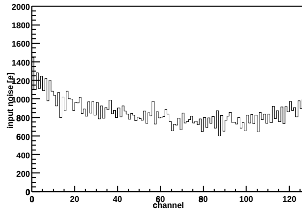
Chip Z36459A-W03-X14-Y03 Input noise vs. channel
