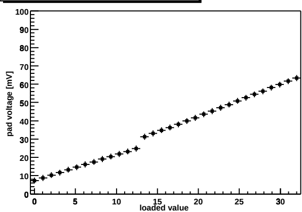
Chip Z36459A-W03-X14-Y03 shaper DAC
