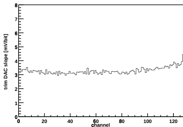
Chip Z36459A-W03-X14-Y03 Trim DAC slope vs. channel
