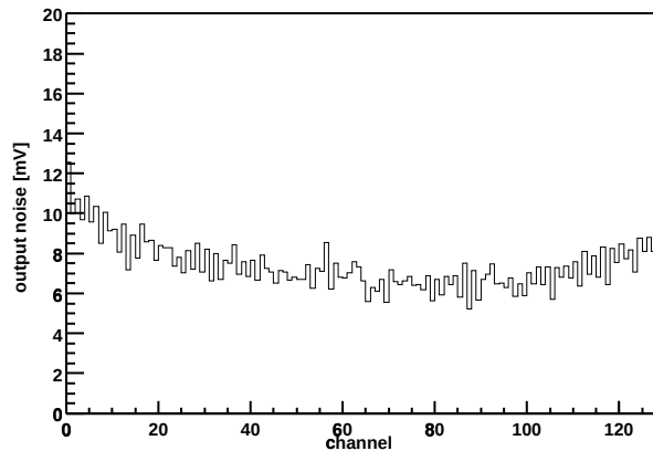
Chip Z36459A-W03-X14-Y03 Output noise vs. channel
