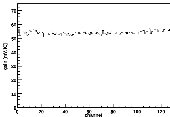
Chip Z36459A-W03-X14-Y03 Gain vs. channel
