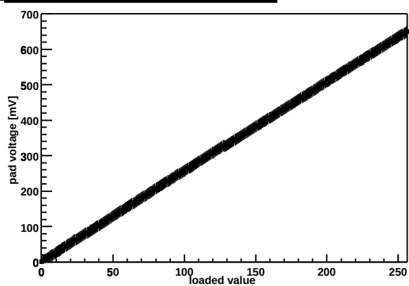
Chip Z36459A-W03-X14-Y03 threshold DAC
