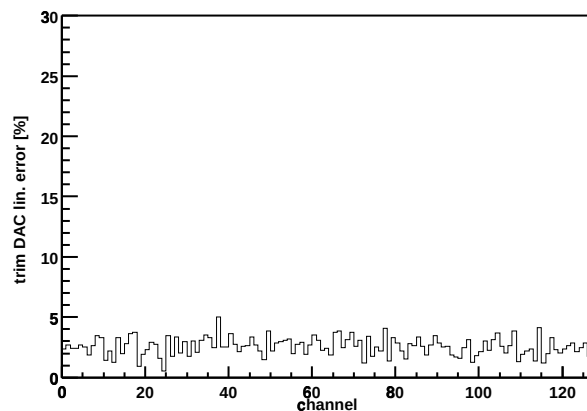
Chip Z36459A-W03-X14-Y03 trim DAC lin. error
