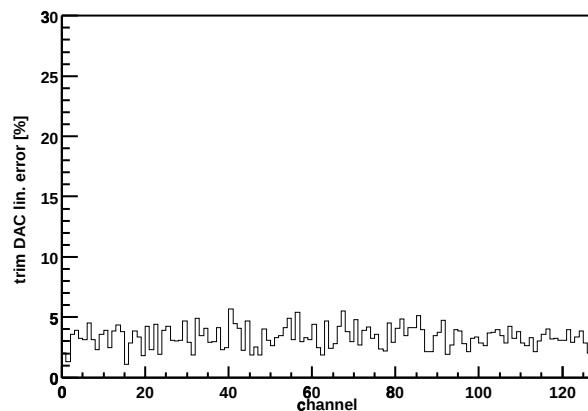
Chip Z36459A-W03-X14-Y10 trim DAC lin. error
