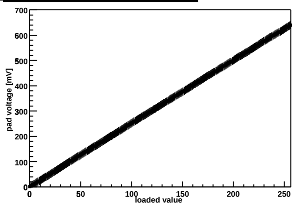
Chip Z36459A-W03-X14-Y10 threshold DAC
