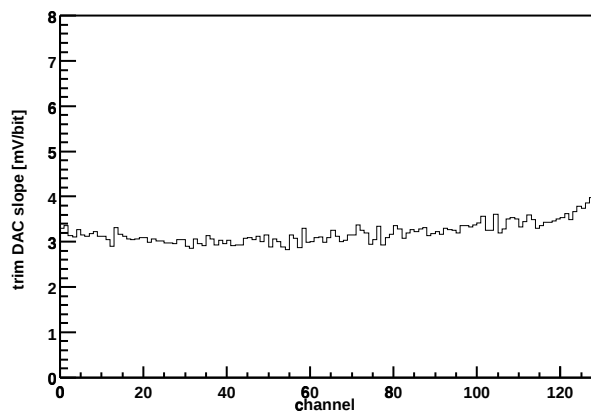
Chip Z36459A-W03-X14-Y10 Trim DAC slope vs. channel
