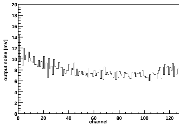
Chip Z36459A-W03-X14-Y10 Output noise vs. channel
