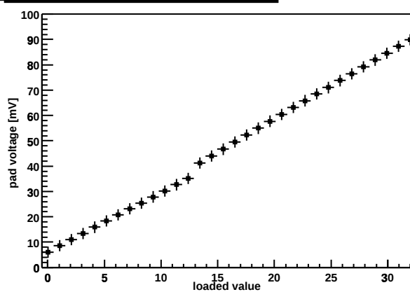
Chip Z36459A-W03-X14-Y10 preamp DAC
