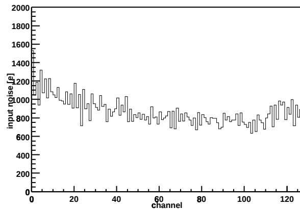
Chip Z36459A-W03-X14-Y10 Input noise vs. channel
