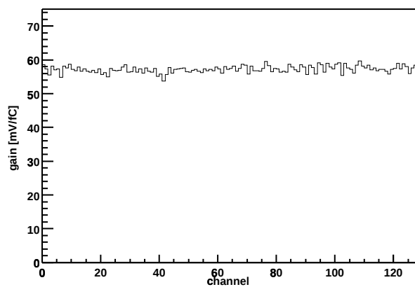
Chip Z36459A-W03-X14-Y10 Gain vs. channel
