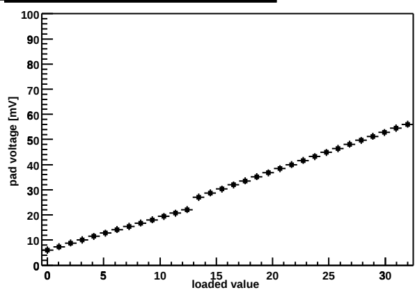
Chip Z36459A-W03-X14-Y10 shaper DAC
