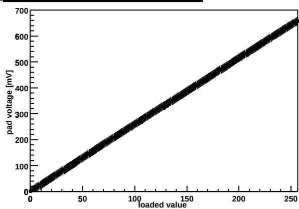
Chip Z36459A-W03-X15-Y06 threshold DAC
