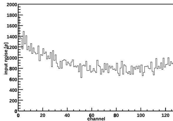
Chip Z36459A-W03-X15-Y06 Input noise vs. channel
