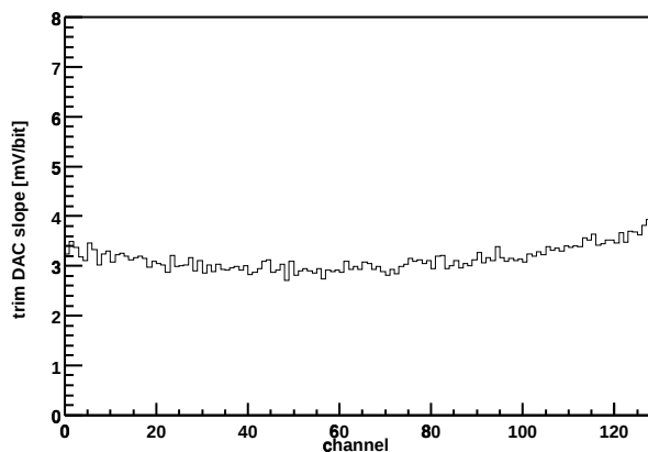
Chip Z36459A-W03-X15-Y06 Trim DAC slope vs. channel
