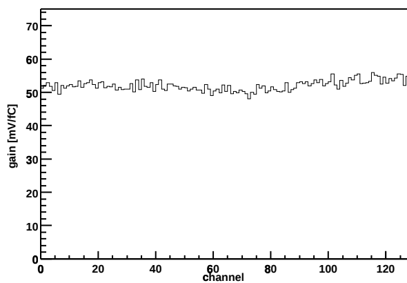
Chip Z36459A-W03-X15-Y06 Gain vs. channel
