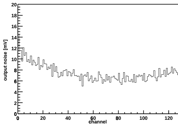
Chip Z36459A-W03-X15-Y06 Output noise vs. channel
