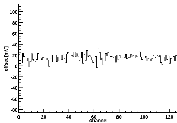
Chip Z36459A-W03-X15-Y06 Offset vs. channel
