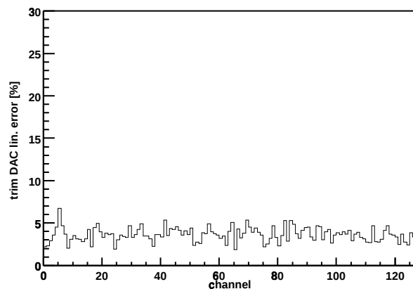
Chip Z36459A-W03-X15-Y06 trim DAC lin. error
