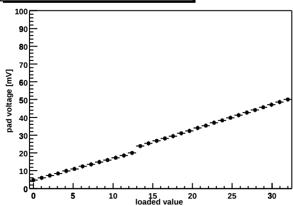
Chip Z36459A-W03-X15-Y06 shaper DAC
