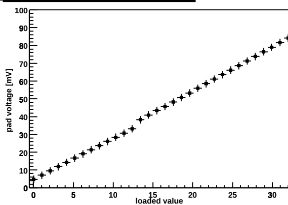
Chip Z36459A-W03-X15-Y06 preamp DAC
