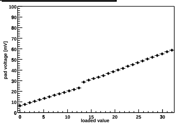
Chip Z36459A-W03-X16-Y07 shaper DAC
