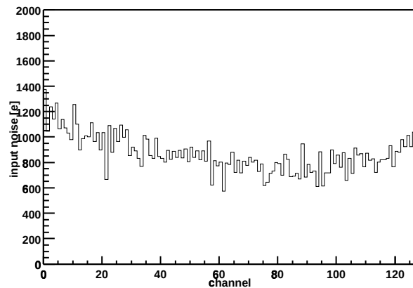
Chip Z36459A-W03-X16-Y07 Input noise vs. channel
