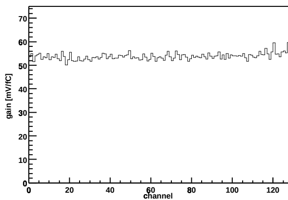
Chip Z36459A-W03-X16-Y07 Gain vs. channel
