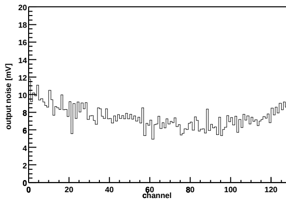
Chip Z36459A-W03-X16-Y07 Output noise vs. channel
