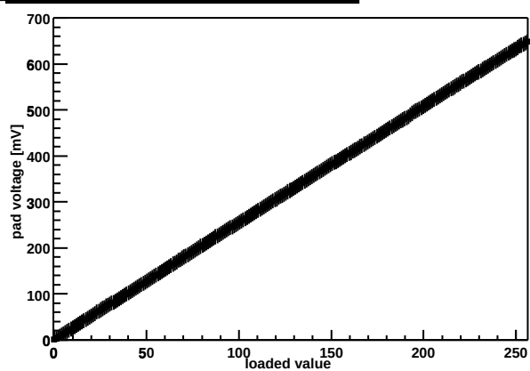
Chip Z36459A-W03-X16-Y07 threshold DAC
