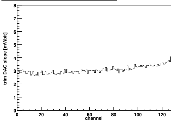
Chip Z36459A-W03-X16-Y07 Trim DAC slope vs. channel
