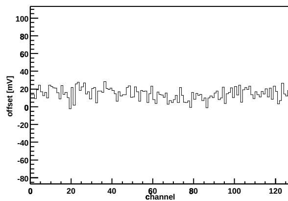
Chip Z36459A-W03-X16-Y07 Offset vs. channel
