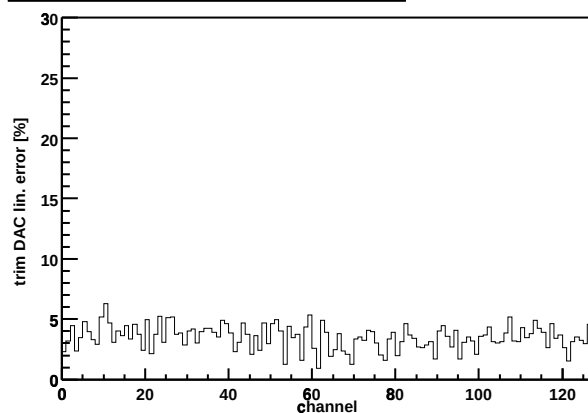
Chip Z36459A-W03-X16-Y07 trim DAC lin. error
