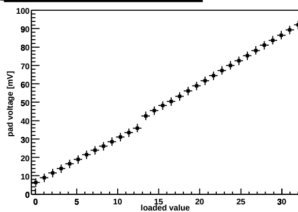
Chip Z36459A-W03-X16-Y07 preamp DAC
