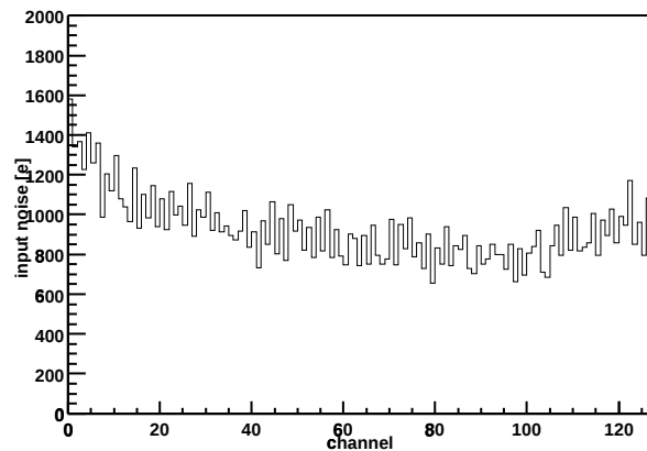
Chip Z36459A-W03-X16-Y08 Input noise vs. channel
