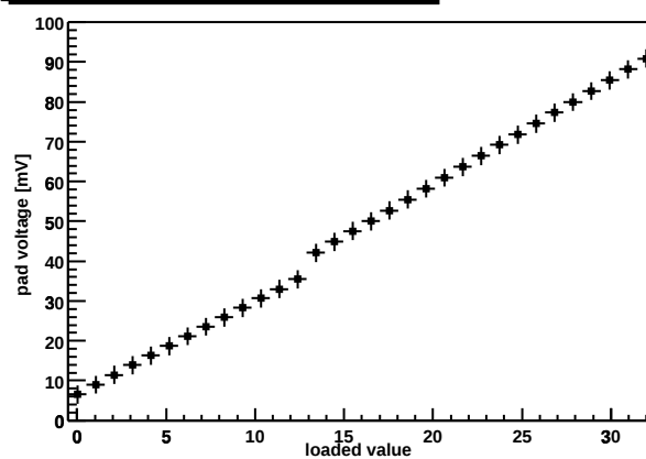
Chip Z36459A-W03-X16-Y08 preamp DAC
