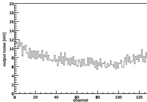
Chip Z36459A-W03-X16-Y08 Output noise vs. channel
