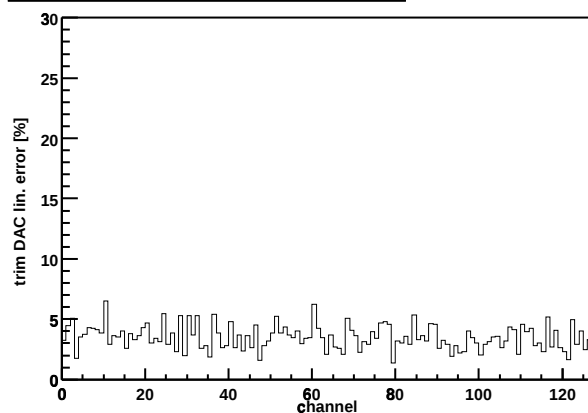
Chip Z36459A-W03-X16-Y08 trim DAC lin. error
