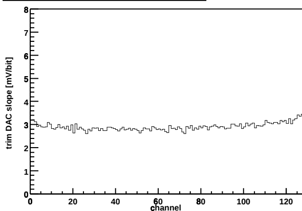
Chip Z36459A-W03-X16-Y08 Trim DAC slope vs. channel
