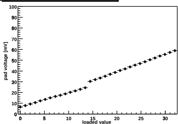
Chip Z36459A-W03-X16-Y08 shaper DAC
