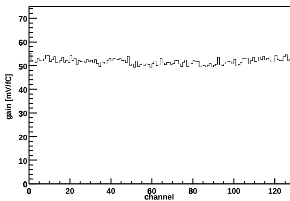
Chip Z36459A-W03-X16-Y08 Gain vs. channel
