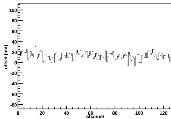
Chip Z36459A-W03-X16-Y08 Offset vs. channel
