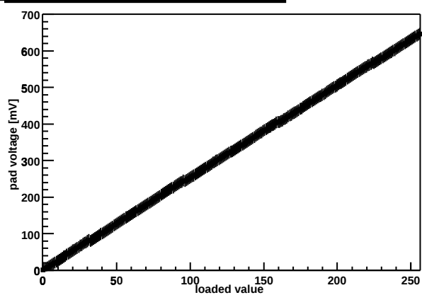
Chip Z36459A-W03-X16-Y08 threshold DAC
