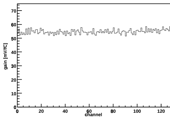
Chip Z36459A-W04-X05-Y01 Gain vs. channel
