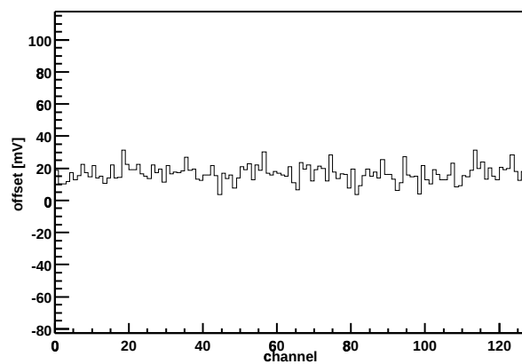
Chip Z36459A-W04-X05-Y01 Offset vs. channel
