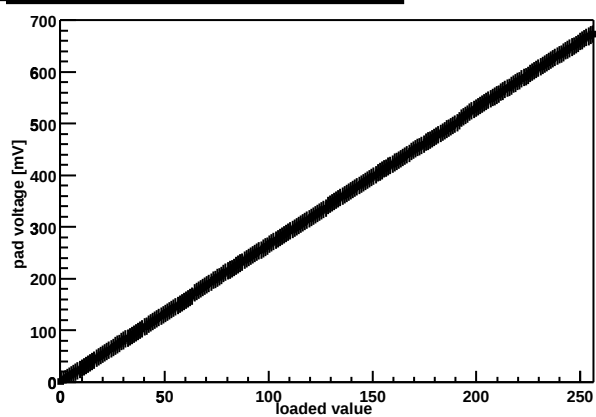
Chip Z36459A-W04-X05-Y01 threshold DAC
