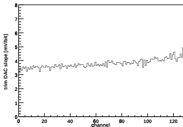
Chip Z36459A-W04-X05-Y01 Trim DAC slope vs. channel
