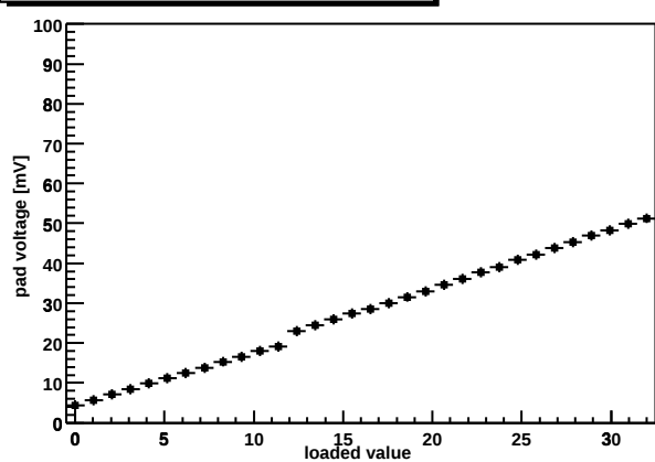
Chip Z36459A-W04-X05-Y01 shaper DAC
