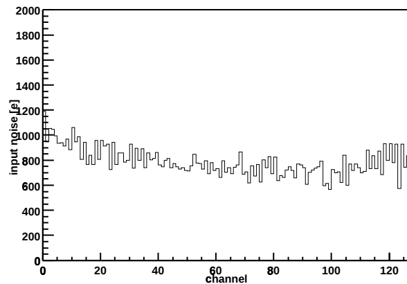
Chip Z36459A-W04-X05-Y01 Input noise vs. channel
