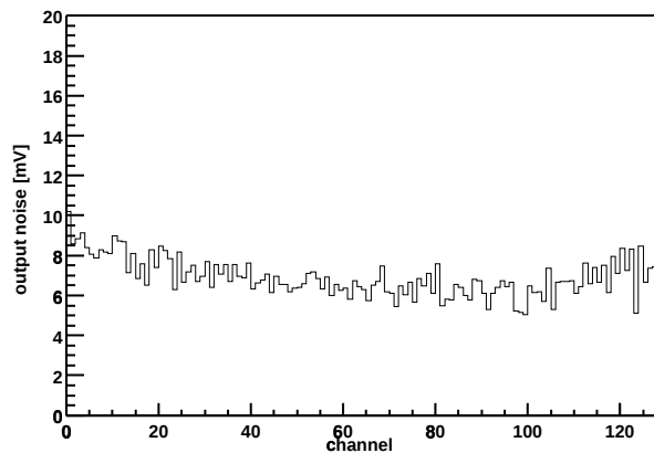
Chip Z36459A-W04-X05-Y01 Output noise vs. channel
