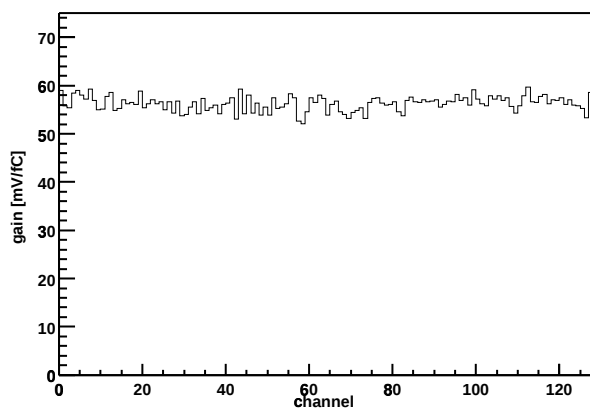
Chip Z36459A-W04-X06-Y06 Gain vs. channel
