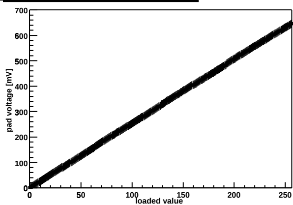
Chip Z36459A-W04-X06-Y06 threshold DAC
