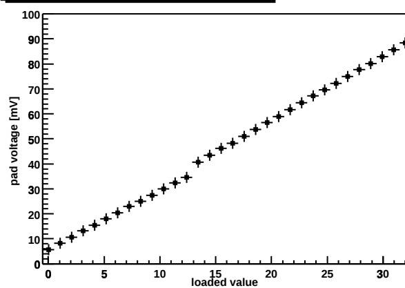
Chip Z36459A-W04-X06-Y06 preamp DAC
