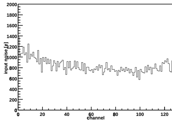
Chip Z36459A-W04-X06-Y06 Input noise vs. channel
