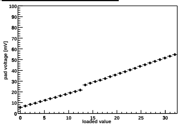
Chip Z36459A-W04-X06-Y06 shaper DAC
