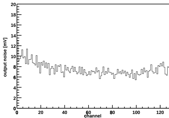
Chip Z36459A-W04-X06-Y06 Output noise vs. channel
