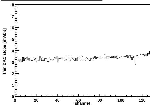
Chip Z36459A-W04-X06-Y06 Trim DAC slope vs. channel
