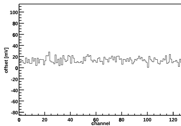
Chip Z36459A-W04-X06-Y06 Offset vs. channel
