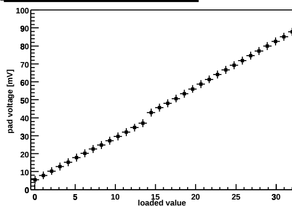
Chip Z36459A-W04-X06-Y09 preamp DAC
