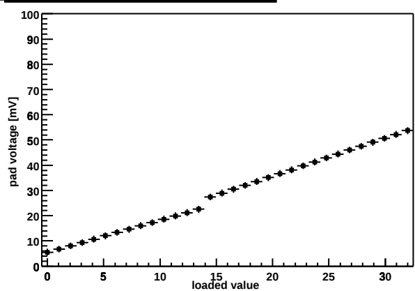
Chip Z36459A-W04-X06-Y09 shaper DAC
