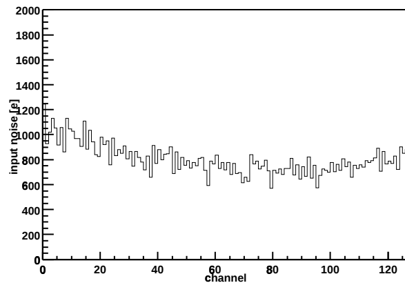
Chip Z36459A-W04-X06-Y09 Input noise vs. channel
