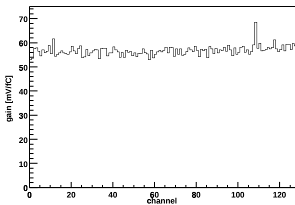
Chip Z36459A-W04-X06-Y09 Gain vs. channel
