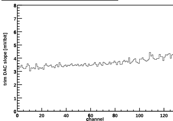
Chip Z36459A-W04-X06-Y09 Trim DAC slope vs. channel
