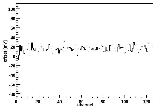
Chip Z36459A-W04-X06-Y09 Offset vs. channel
