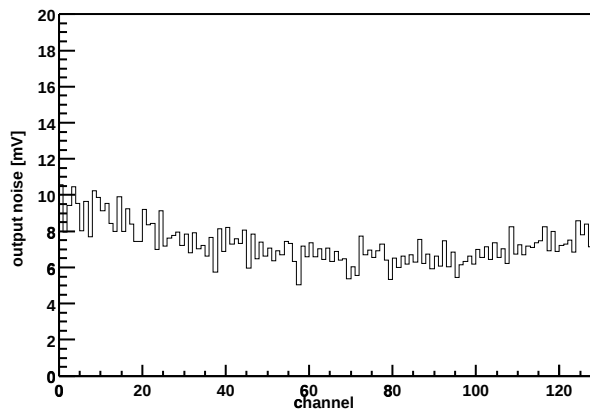
Chip Z36459A-W04-X06-Y09 Output noise vs. channel
