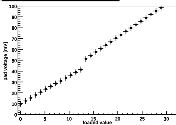
Chip Z36459A-W04-X06-Y10 preamp DAC
