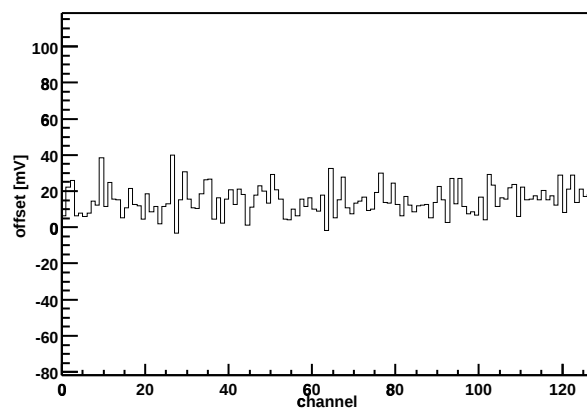
Chip Z36459A-W04-X06-Y10 Offset vs. channel
