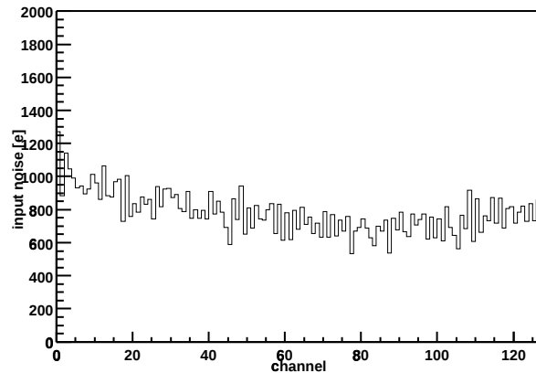
Chip Z36459A-W04-X06-Y10 Input noise vs. channel
