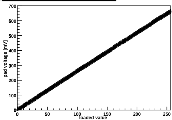
Chip Z36459A-W04-X06-Y10 threshold DAC
