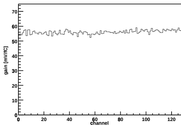
Chip Z36459A-W04-X06-Y10 Gain vs. channel
