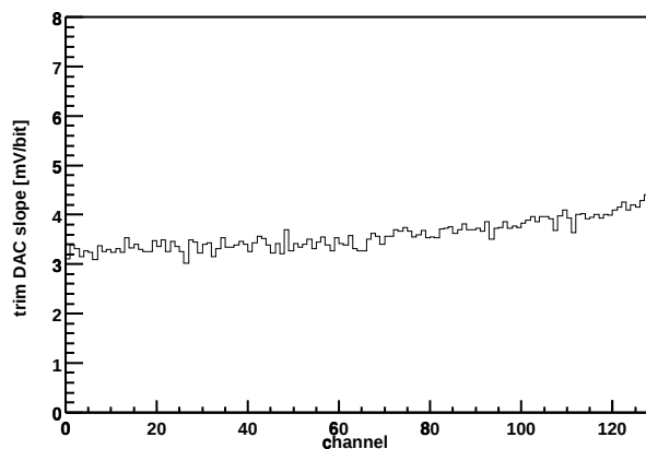
Chip Z36459A-W04-X06-Y10 Trim DAC slope vs. channel
