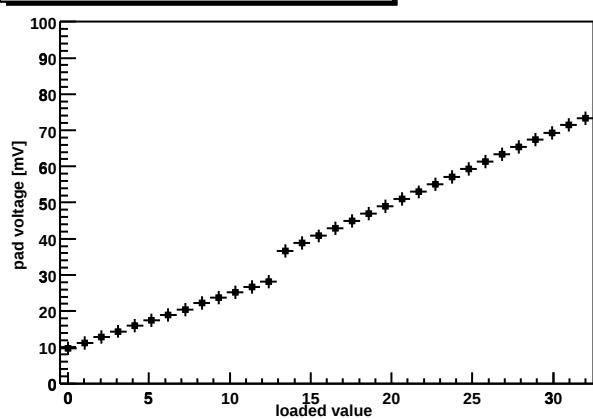
Chip Z36459A-W04-X06-Y10 shaper DAC
