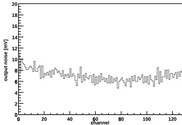
Chip Z36459A-W04-X06-Y10 Output noise vs. channel
