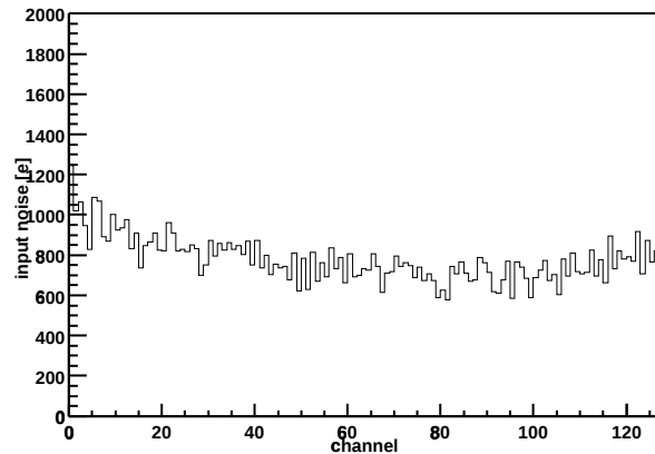
Chip Z36459A-W04-X06-Y13 Input noise vs. channel
