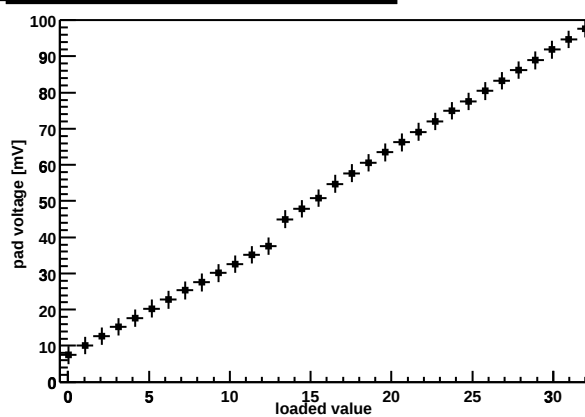
Chip Z36459A-W04-X06-Y13 preamp DAC
