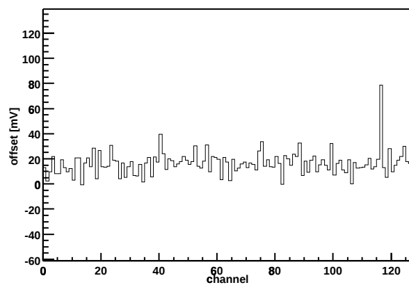
Chip Z36459A-W04-X06-Y13 Offset vs. channel
