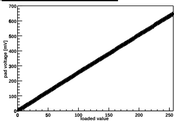
Chip Z36459A-W04-X06-Y13 threshold DAC
