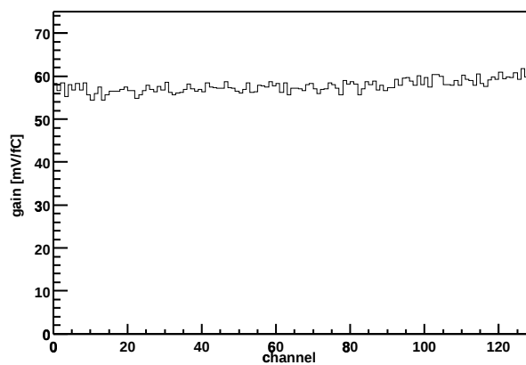
Chip Z36459A-W04-X06-Y13 Gain vs. channel
