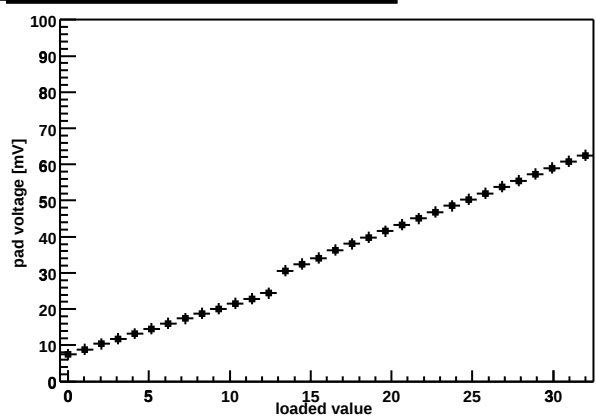
Chip Z36459A-W04-X06-Y13 shaper DAC
