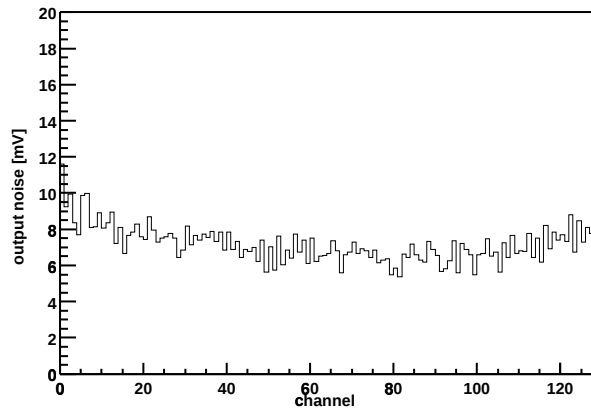
Chip Z36459A-W04-X06-Y13 Output noise vs. channel
