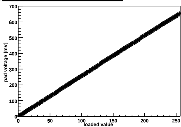
Chip Z36459A-W04-X07-Y06 threshold DAC
