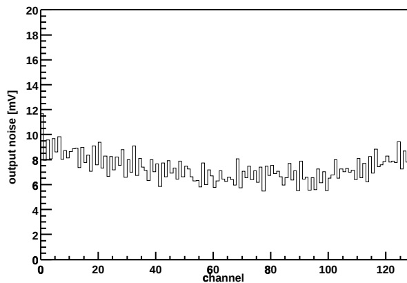
Chip Z36459A-W04-X07-Y06 Output noise vs. channel
