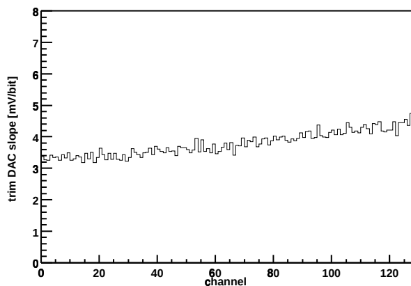
Chip Z36459A-W04-X07-Y06 Trim DAC slope vs. channel
