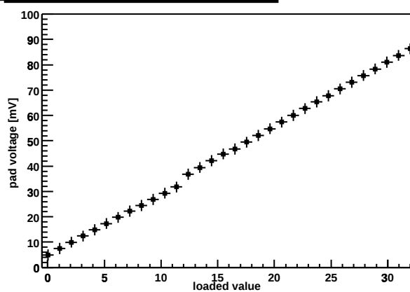
Chip Z36459A-W04-X07-Y06 preamp DAC
