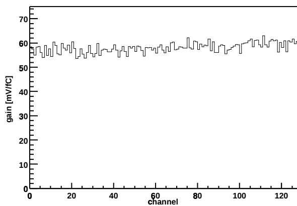
Chip Z36459A-W04-X07-Y06 Gain vs. channel
