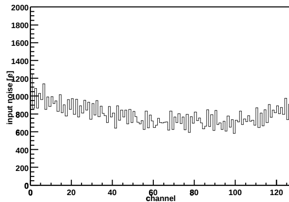
Chip Z36459A-W04-X07-Y06 Input noise vs. channel
