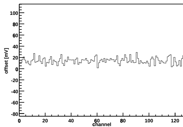
Chip Z36459A-W04-X07-Y06 Offset vs. channel
