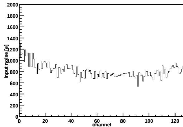
Chip Z36459A-W04-X07-Y07 Input noise vs. channel
