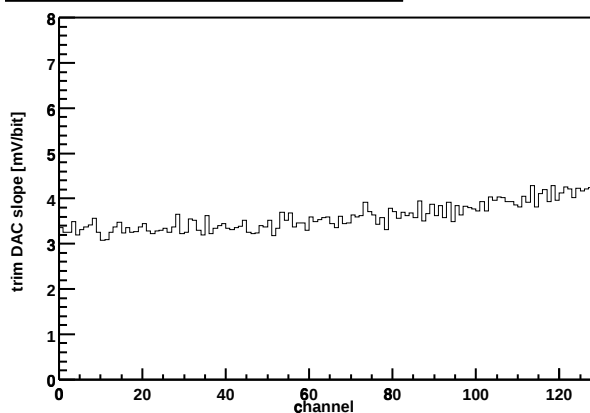
Chip Z36459A-W04-X07-Y07 Trim DAC slope vs. channel
