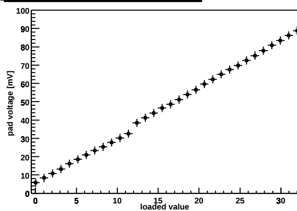
Chip Z36459A-W04-X07-Y07 preamp DAC
