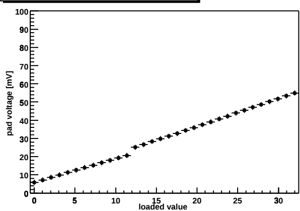
Chip Z36459A-W04-X07-Y07 shaper DAC
