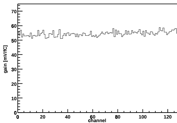
Chip Z36459A-W04-X07-Y07 Gain vs. channel
