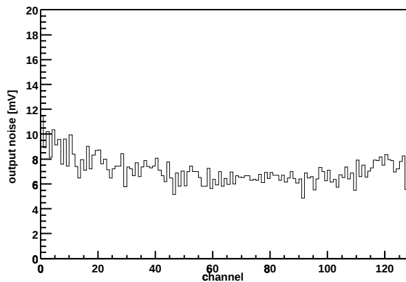
Chip Z36459A-W04-X07-Y07 Output noise vs. channel
