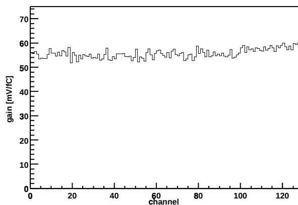
Chip Z36459A-W04-X07-Y08 Gain vs. channel
