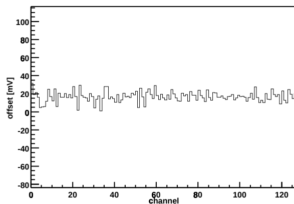
Chip Z36459A-W04-X07-Y08 Offset vs. channel
