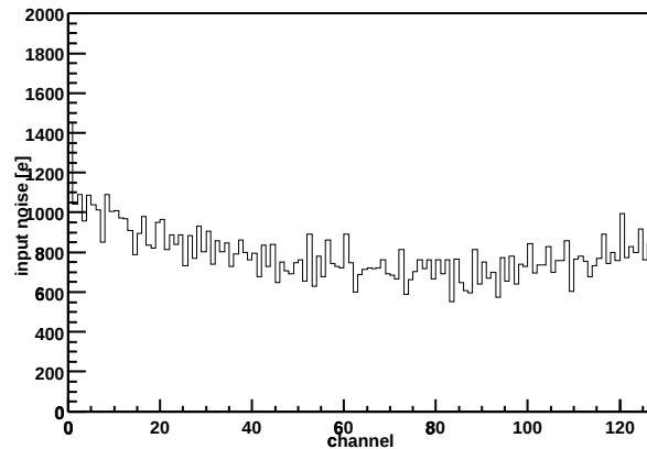
Chip Z36459A-W04-X07-Y08 Input noise vs. channel
