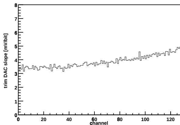
Chip Z36459A-W04-X07-Y08 Trim DAC slope vs. channel
