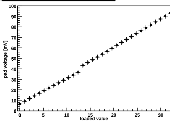
Chip Z36459A-W04-X07-Y08 preamp DAC
