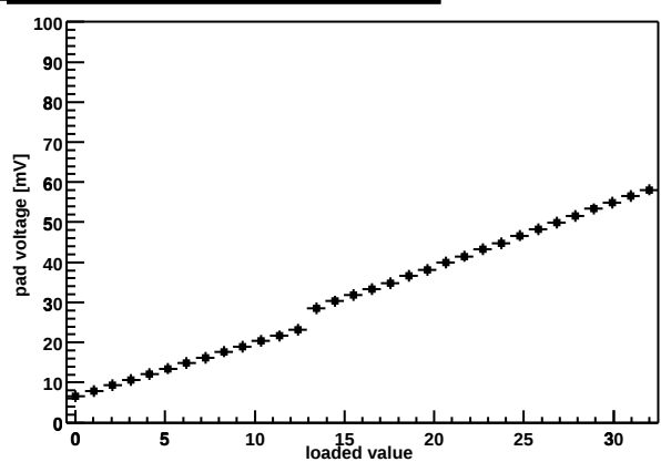
Chip Z36459A-W04-X07-Y08 shaper DAC
