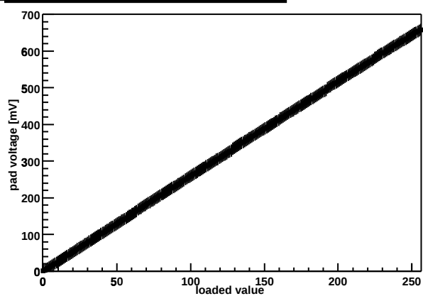
Chip Z36459A-W04-X07-Y08 threshold DAC
