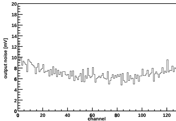
Chip Z36459A-W04-X07-Y08 Output noise vs. channel
