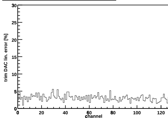
Chip Z36459A-W04-X07-Y12 trim DAC lin. error
