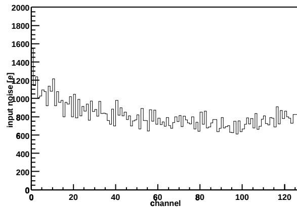
Chip Z36459A-W04-X07-Y12 Input noise vs. channel
