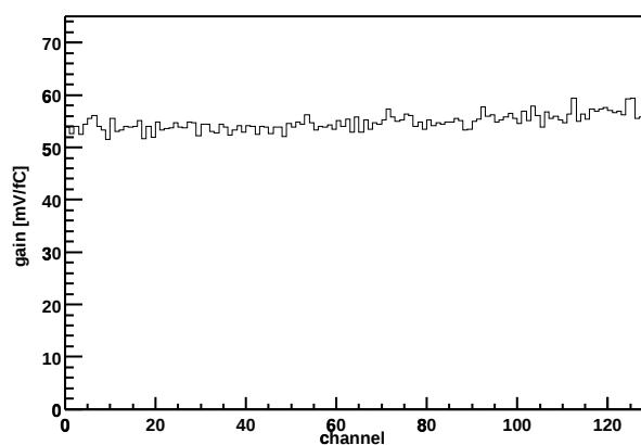
Chip Z36459A-W04-X07-Y12 Gain vs. channel
