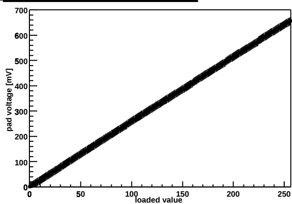
Chip Z36459A-W04-X07-Y12 threshold DAC
