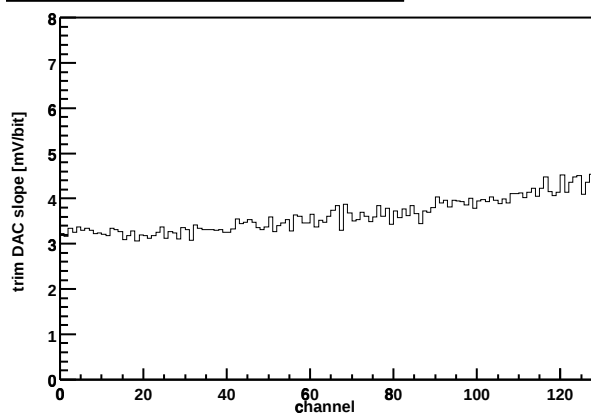
Chip Z36459A-W04-X07-Y12 Trim DAC slope vs. channel
