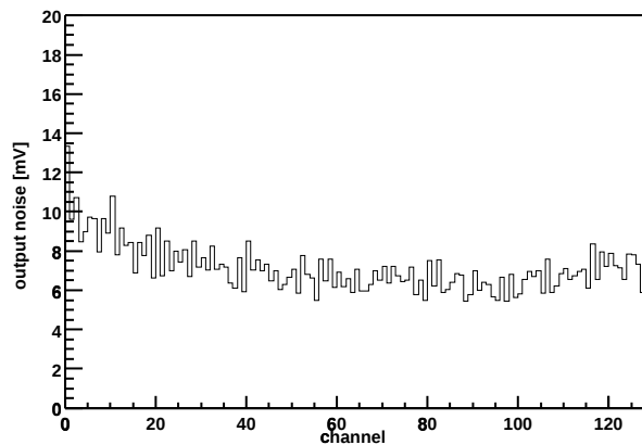
Chip Z36459A-W04-X07-Y12 Output noise vs. channel
