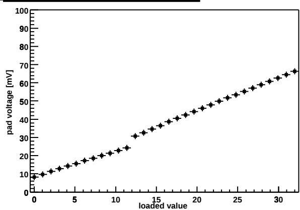
Chip Z36459A-W04-X07-Y12 shaper DAC
