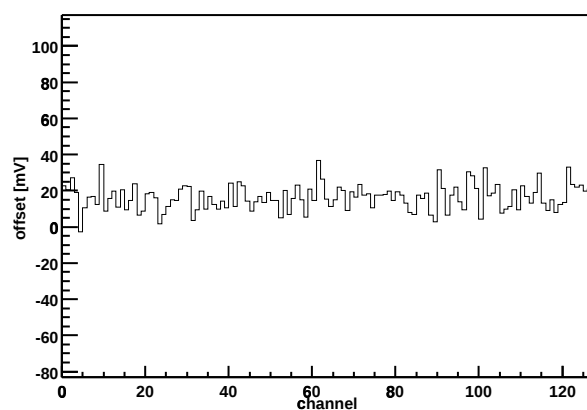
Chip Z36459A-W04-X07-Y12 Offset vs. channel
