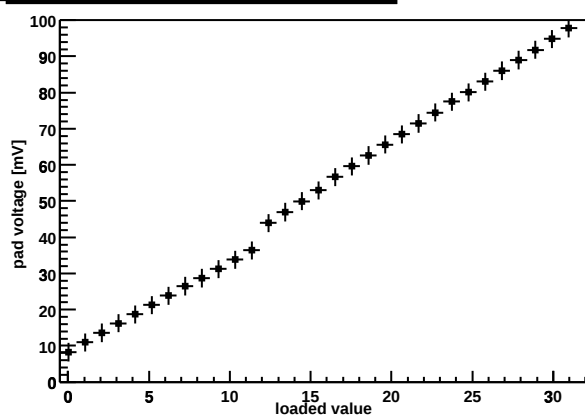
Chip Z36459A-W04-X07-Y12 preamp DAC
