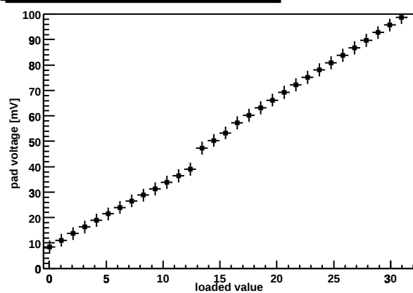
Chip Z36459A-W04-X07-Y16 preamp DAC
