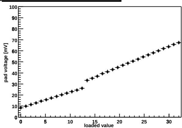
Chip Z36459A-W04-X07-Y16 shaper DAC
