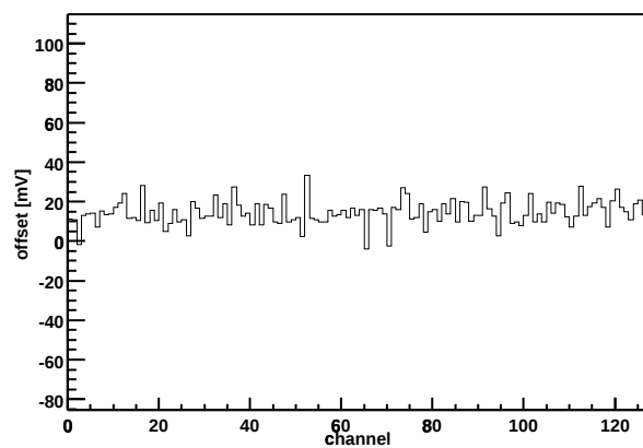
Chip Z36459A-W04-X07-Y16 Offset vs. channel
