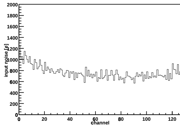
Chip Z36459A-W04-X07-Y16 Input noise vs. channel
