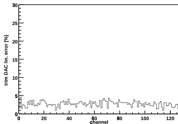
Chip Z36459A-W04-X07-Y16 trim DAC lin. error
