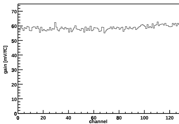
Chip Z36459A-W04-X07-Y16 Gain vs. channel
