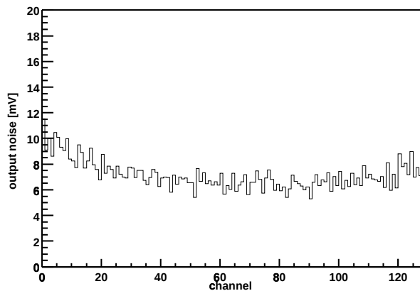
Chip Z36459A-W04-X07-Y16 Output noise vs. channel
