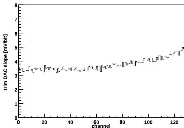
Chip Z36459A-W04-X07-Y16 Trim DAC slope vs. channel
