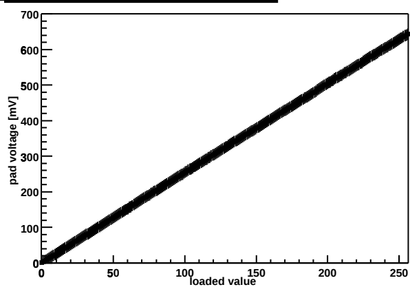
Chip Z36459A-W04-X07-Y16 threshold DAC
