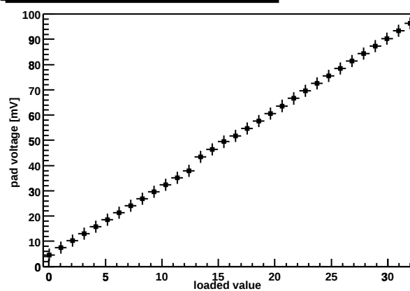
Chip Z36459A-W04-X08-Y00 preamp DAC
