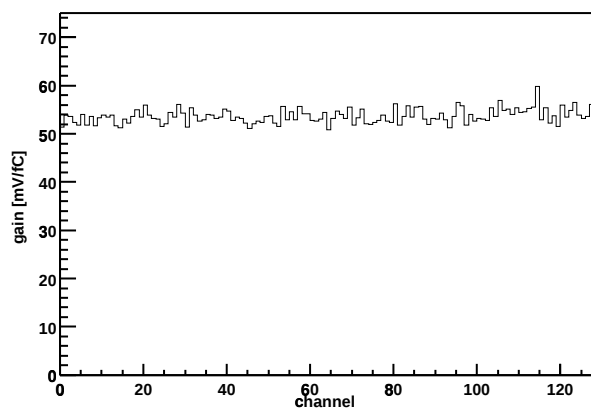
Chip Z36459A-W04-X08-Y00 Gain vs. channel
