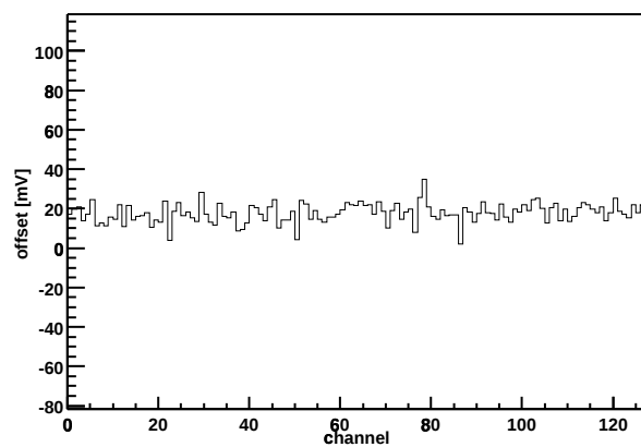
Chip Z36459A-W04-X08-Y00 Offset vs. channel
