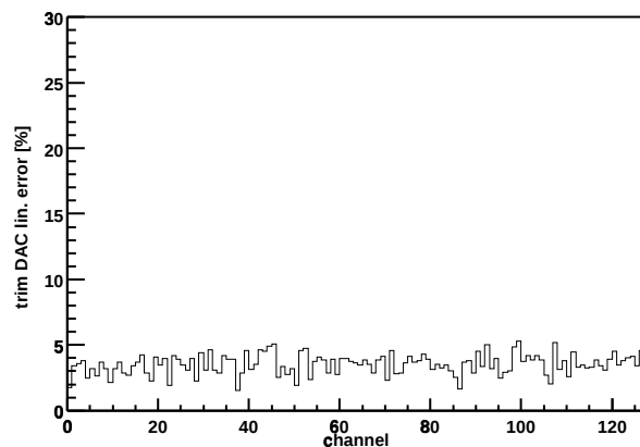
Chip Z36459A-W04-X08-Y00 trim DAC lin. error
