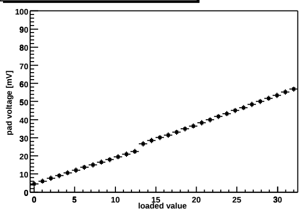
Chip Z36459A-W04-X08-Y00 shaper DAC
