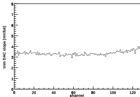
Chip Z36459A-W04-X08-Y00 Trim DAC slope vs. channel
