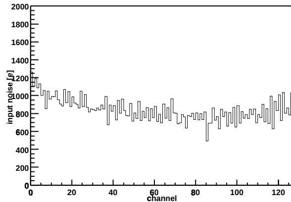
Chip Z36459A-W04-X08-Y00 Input noise vs. channel
