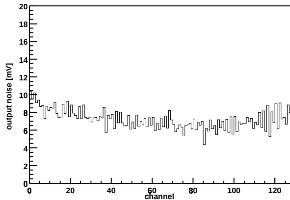
Chip Z36459A-W04-X08-Y00 Output noise vs. channel
