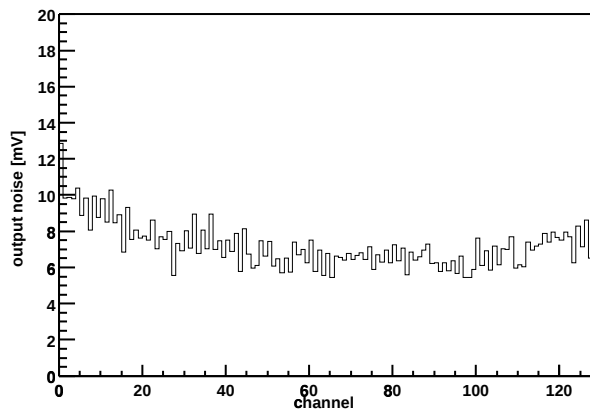
Chip Z36459A-W04-X08-Y12 Output noise vs. channel
