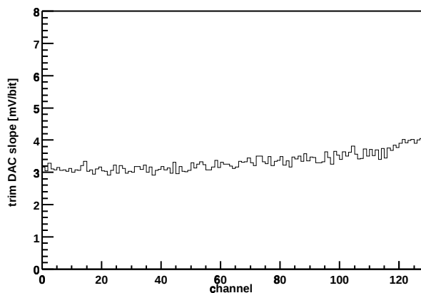
Chip Z36459A-W04-X08-Y12 Trim DAC slope vs. channel
