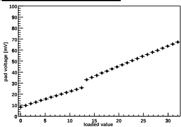
Chip Z36459A-W04-X08-Y12 shaper DAC
