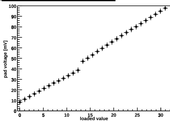
Chip Z36459A-W04-X08-Y12 preamp DAC
