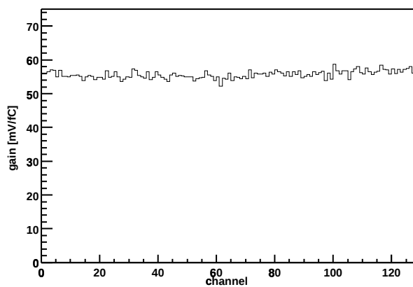
Chip Z36459A-W04-X08-Y12 Gain vs. channel
