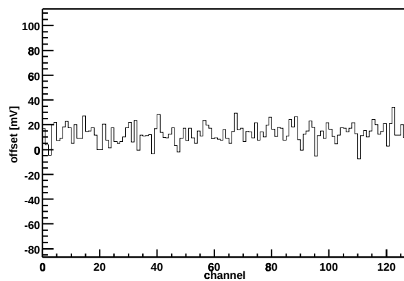
Chip Z36459A-W04-X08-Y12 Offset vs. channel
