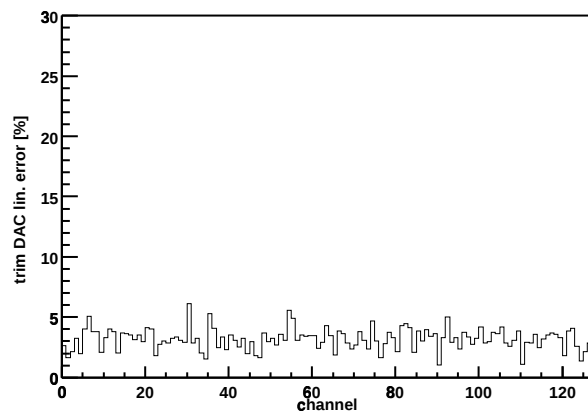
Chip Z36459A-W04-X08-Y12 trim DAC lin. error
