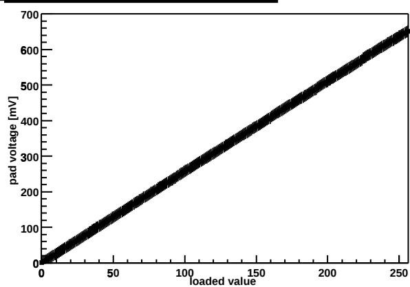
Chip Z36459A-W04-X08-Y12 threshold DAC
