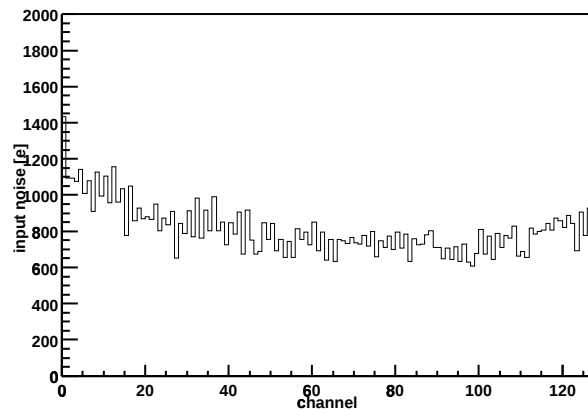
Chip Z36459A-W04-X08-Y12 Input noise vs. channel
