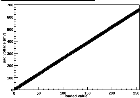
Chip Z36459A-W04-X08-Y13 threshold DAC
