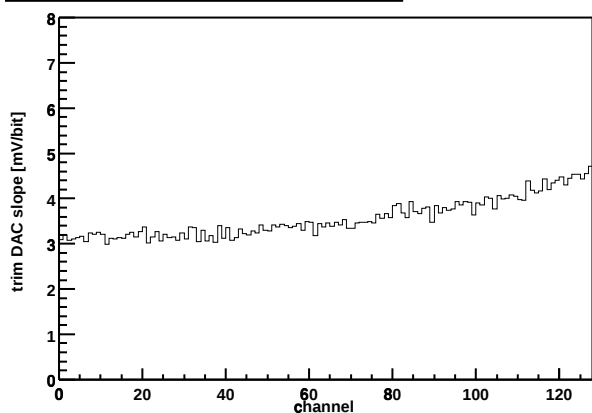
Chip Z36459A-W04-X08-Y13 Trim DAC slope vs. channel
