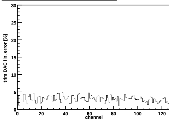
Chip Z36459A-W04-X08-Y13 trim DAC lin. error
