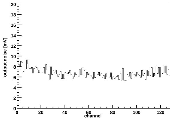
Chip Z36459A-W04-X08-Y13 Output noise vs. channel
