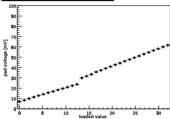
Chip Z36459A-W04-X08-Y13 shaper DAC
