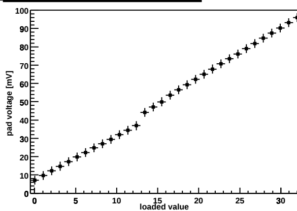
Chip Z36459A-W04-X08-Y13 preamp DAC
