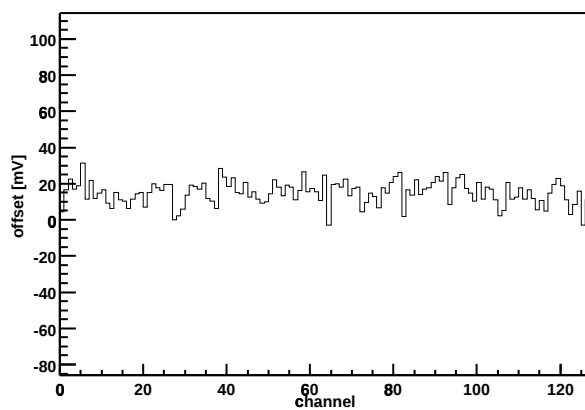
Chip Z36459A-W04-X08-Y13 Offset vs. channel
