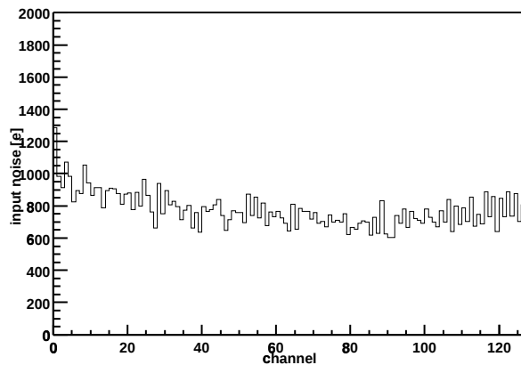
Chip Z36459A-W04-X08-Y13 Input noise vs. channel
