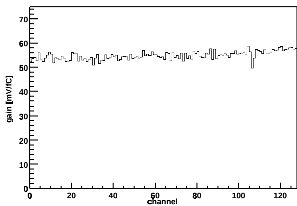
Chip Z36459A-W04-X08-Y13 Gain vs. channel
