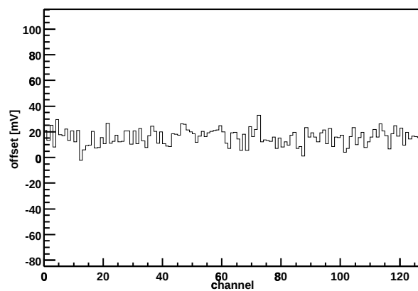
Chip Z36459A-W04-X08-Y18 Offset vs. channel
