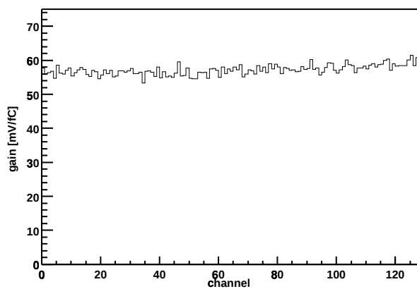
Chip Z36459A-W04-X08-Y18 Gain vs. channel
