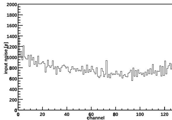
Chip Z36459A-W04-X08-Y18 Input noise vs. channel
