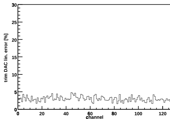
Chip Z36459A-W04-X08-Y18 trim DAC lin. error
