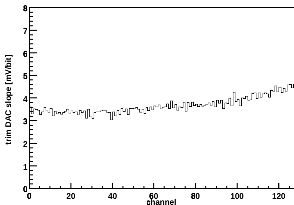
Chip Z36459A-W04-X08-Y18 Trim DAC slope vs. channel
