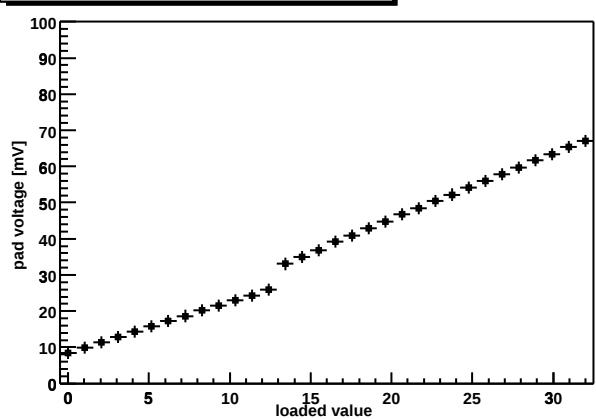
Chip Z36459A-W04-X08-Y18 shaper DAC
