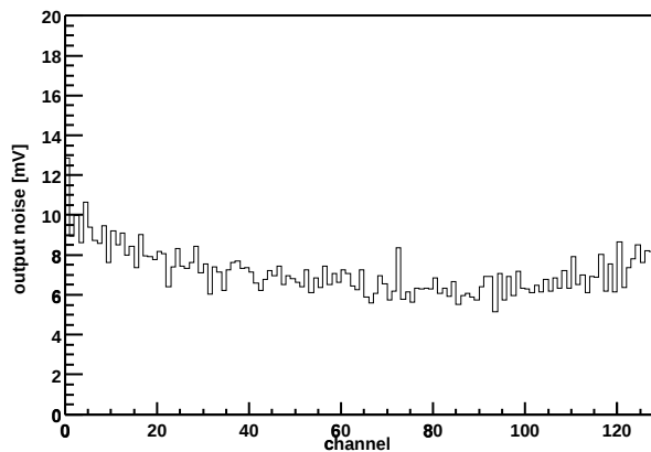
Chip Z36459A-W04-X08-Y18 Output noise vs. channel
