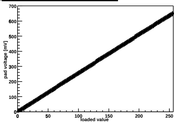
Chip Z36459A-W04-X09-Y08 threshold DAC
