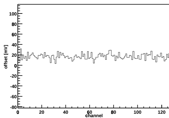
Chip Z36459A-W04-X09-Y08 Offset vs. channel
