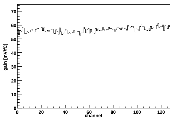
Chip Z36459A-W04-X09-Y08 Gain vs. channel
