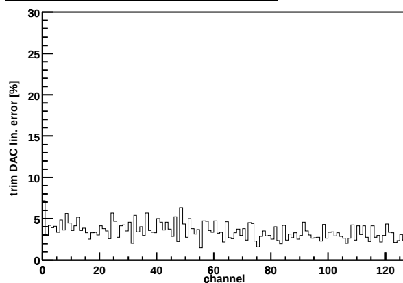
Chip Z36459A-W04-X09-Y08 trim DAC lin. error
