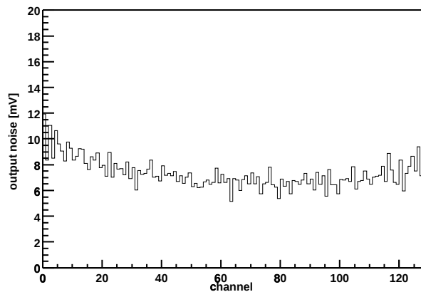
Chip Z36459A-W04-X09-Y08 Output noise vs. channel
