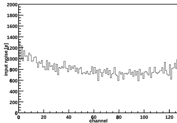
Chip Z36459A-W04-X09-Y08 Input noise vs. channel
