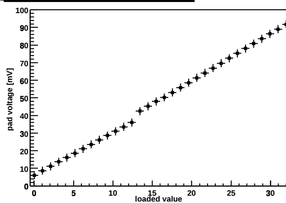
Chip Z36459A-W04-X09-Y08 preamp DAC
