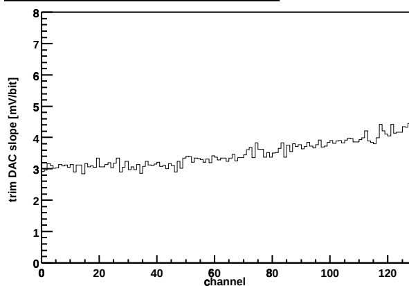
Chip Z36459A-W04-X09-Y08 Trim DAC slope vs. channel
