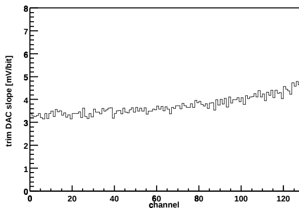
Chip Z36459A-W04-X09-Y13 Trim DAC slope vs. channel
