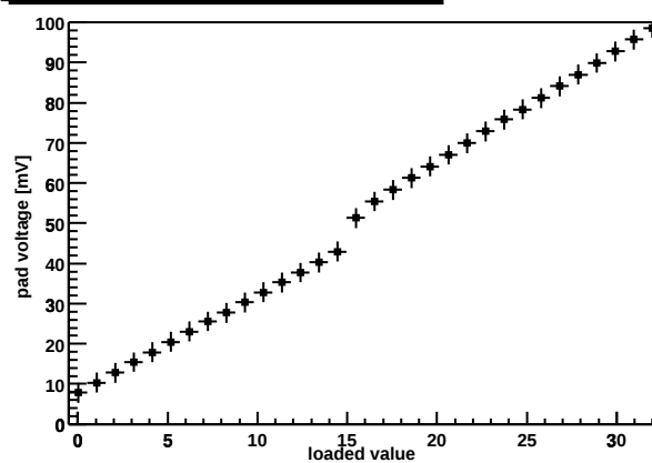
Chip Z36459A-W04-X09-Y13 preamp DAC
