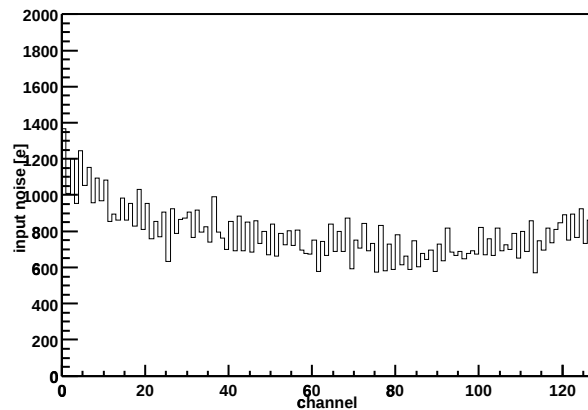
Chip Z36459A-W04-X09-Y13 Input noise vs. channel
