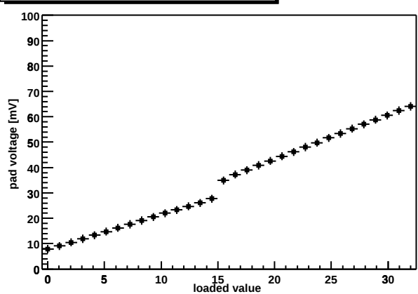
Chip Z36459A-W04-X09-Y13 shaper DAC
