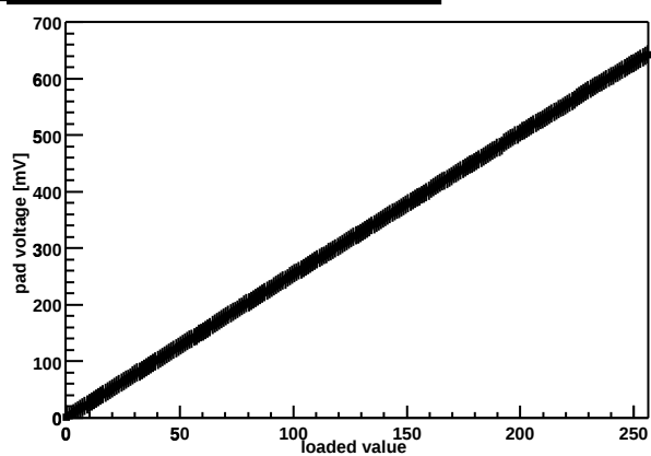
Chip Z36459A-W04-X09-Y13 threshold DAC
