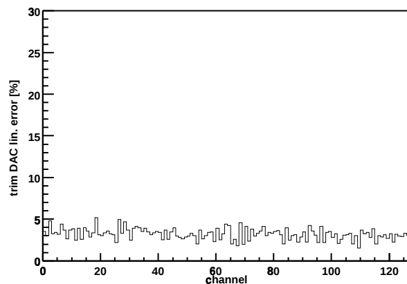
Chip Z36459A-W04-X09-Y13 trim DAC lin. error
