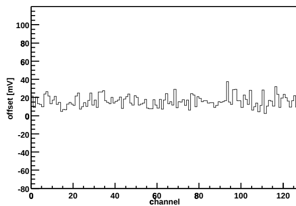
Chip Z36459A-W04-X09-Y13 Offset vs. channel
