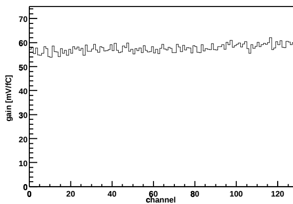
Chip Z36459A-W04-X09-Y13 Gain vs. channel
