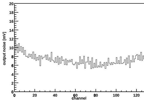
Chip Z36459A-W04-X09-Y13 Output noise vs. channel
