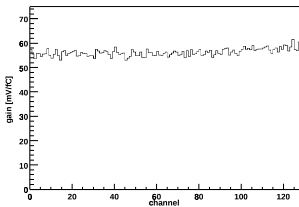
Chip Z36459A-W04-X09-Y14 Gain vs. channel
