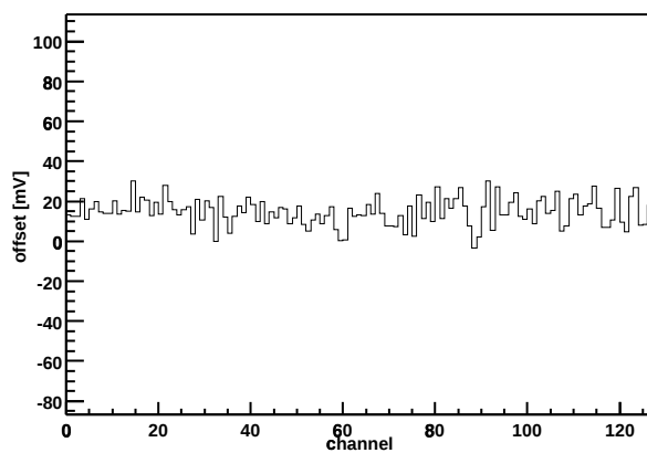
Chip Z36459A-W04-X09-Y14 Offset vs. channel
