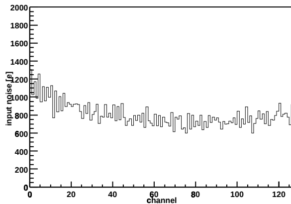
Chip Z36459A-W04-X09-Y14 Input noise vs. channel
