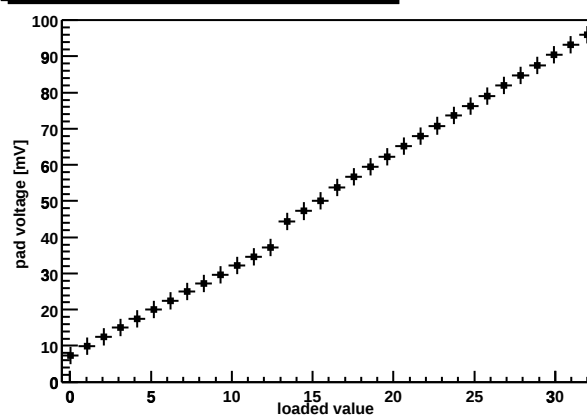
Chip Z36459A-W04-X09-Y14 preamp DAC
