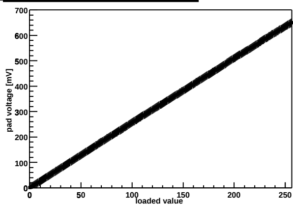
Chip Z36459A-W04-X09-Y14 threshold DAC
