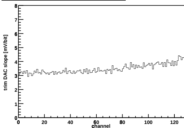
Chip Z36459A-W04-X09-Y14 Trim DAC slope vs. channel
