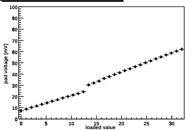
Chip Z36459A-W04-X09-Y14 shaper DAC
