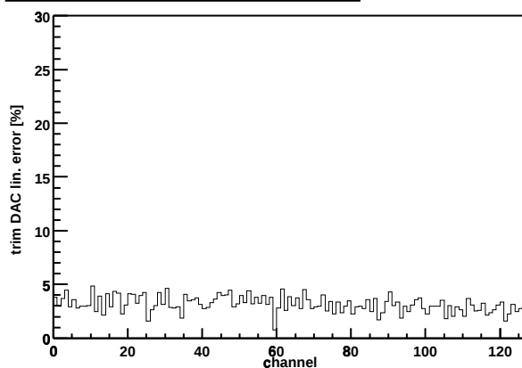
Chip Z36459A-W04-X09-Y14 trim DAC lin. error
