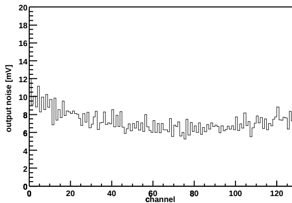
Chip Z36459A-W04-X09-Y14 Output noise vs. channel
