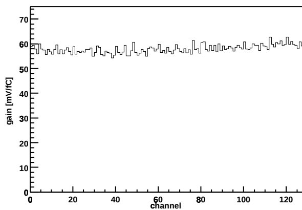
Chip Z36459A-W04-X09-Y17 Gain vs. channel
