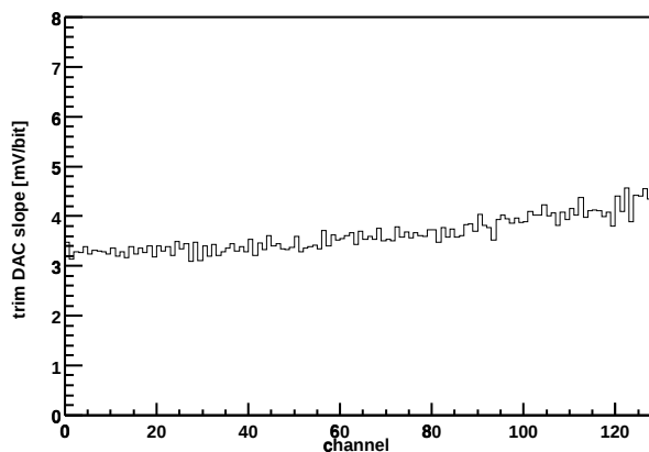
Chip Z36459A-W04-X09-Y17 Trim DAC slope vs. channel
