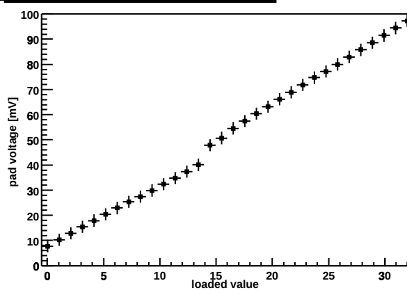
Chip Z36459A-W04-X09-Y17 preamp DAC
