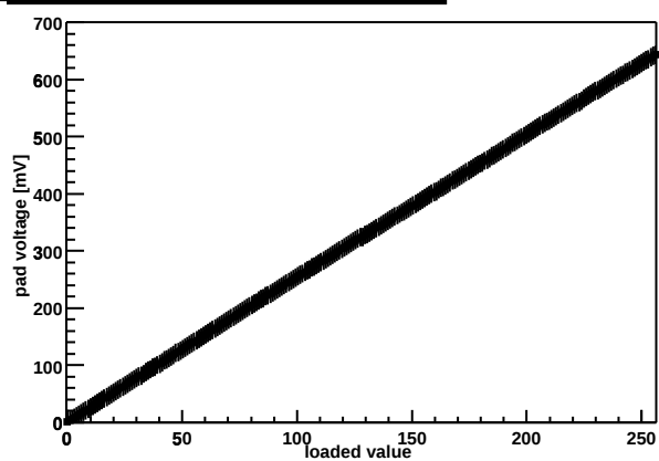
Chip Z36459A-W04-X09-Y17 threshold DAC
