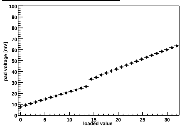
Chip Z36459A-W04-X09-Y17 shaper DAC
