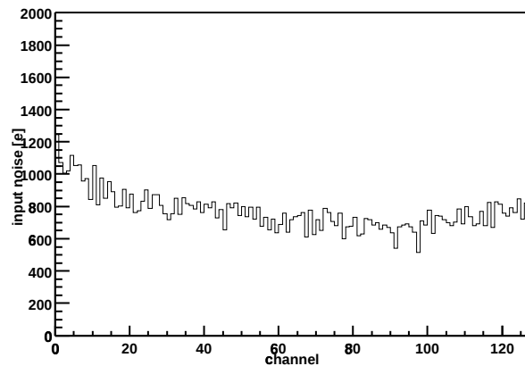
Chip Z36459A-W04-X09-Y17 Input noise vs. channel
