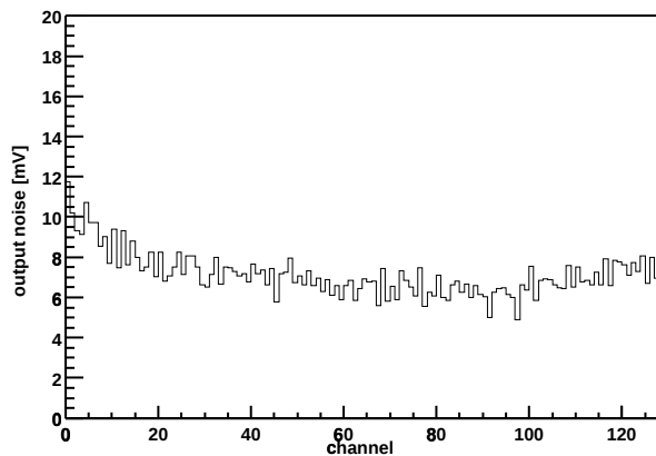
Chip Z36459A-W04-X09-Y17 Output noise vs. channel
