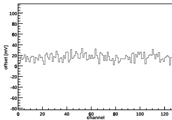
Chip Z36459A-W04-X09-Y17 Offset vs. channel
