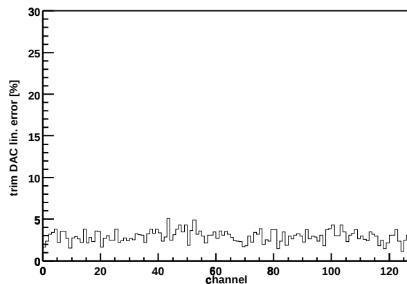
Chip Z36459A-W04-X09-Y17 trim DAC lin. error
