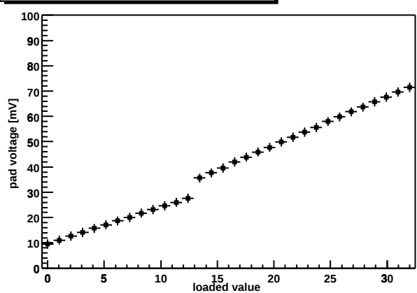
Chip Z36459A-W04-X10-Y13 shaper DAC
