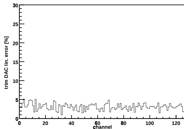
Chip Z36459A-W04-X10-Y13 trim DAC lin. error
