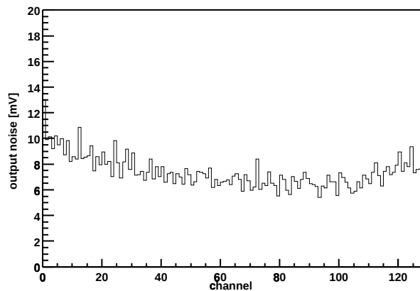
Chip Z36459A-W04-X10-Y13 Output noise vs. channel
