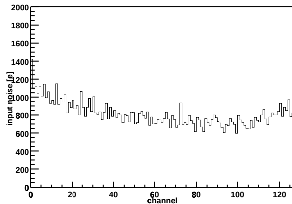
Chip Z36459A-W04-X10-Y13 Input noise vs. channel
