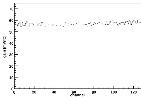
Chip Z36459A-W04-X10-Y13 Gain vs. channel
