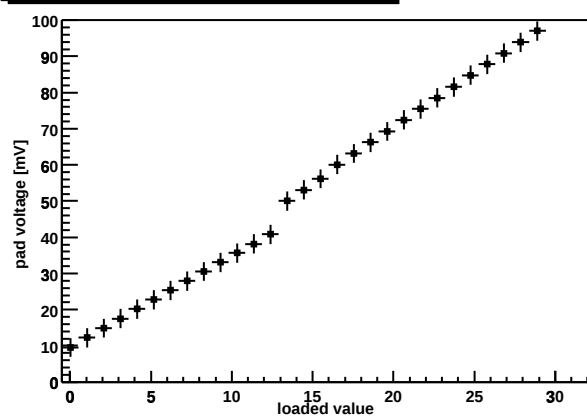
Chip Z36459A-W04-X10-Y13 preamp DAC
