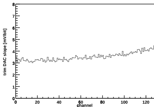
Chip Z36459A-W04-X10-Y13 Trim DAC slope vs. channel
