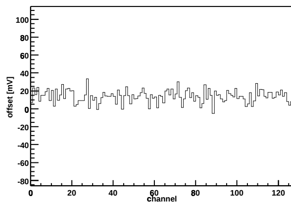
Chip Z36459A-W04-X10-Y13 Offset vs. channel
