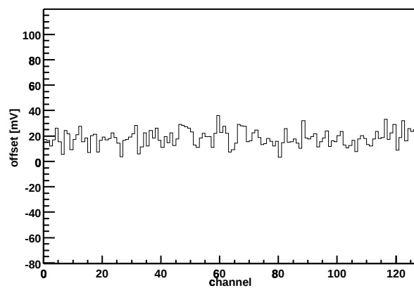
Chip Z36459A-W04-X10-Y19 Offset vs. channel
