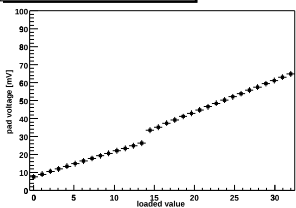
Chip Z36459A-W04-X10-Y19 shaper DAC
