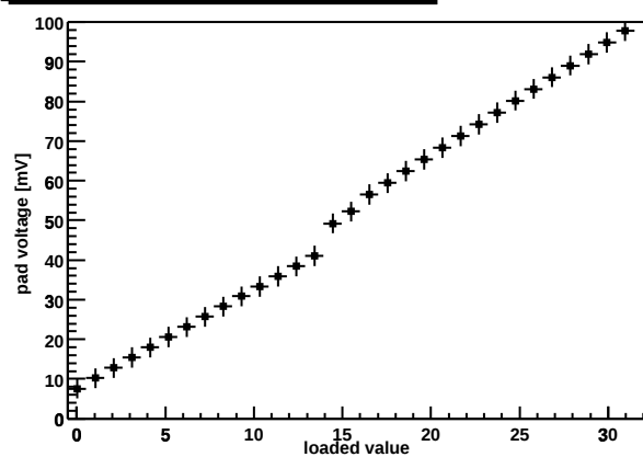
Chip Z36459A-W04-X10-Y19 preamp DAC
