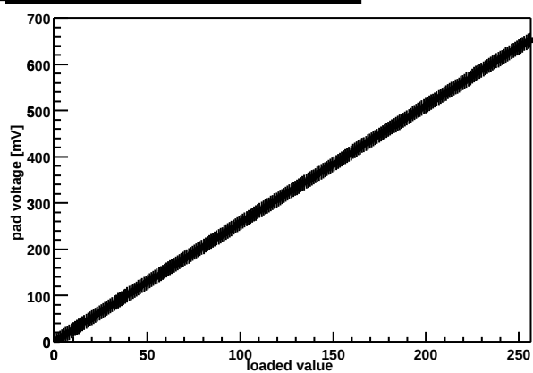
Chip Z36459A-W04-X10-Y19 threshold DAC
