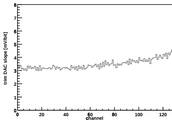
Chip Z36459A-W04-X10-Y19 Trim DAC slope vs. channel
