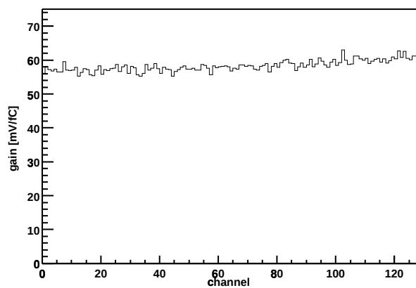
Chip Z36459A-W04-X10-Y19 Gain vs. channel
