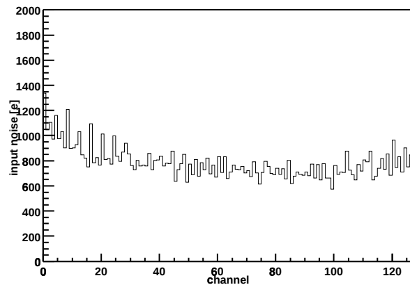
Chip Z36459A-W04-X10-Y19 Input noise vs. channel
