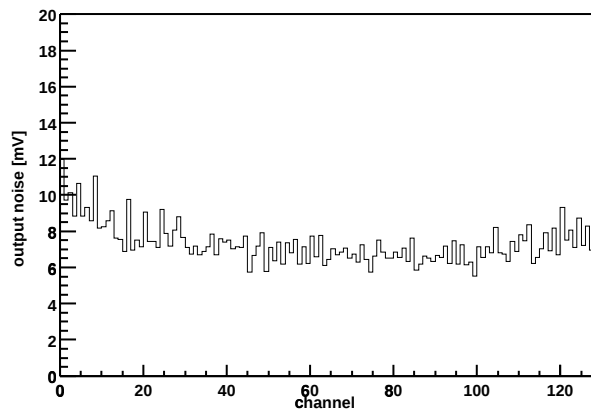
Chip Z36459A-W04-X10-Y19 Output noise vs. channel
