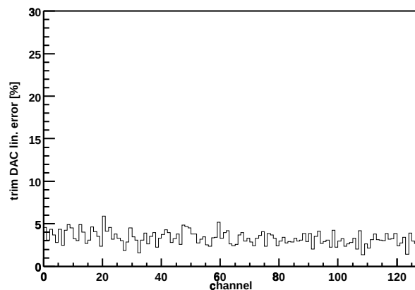
Chip Z36459A-W04-X10-Y19 trim DAC lin. error
