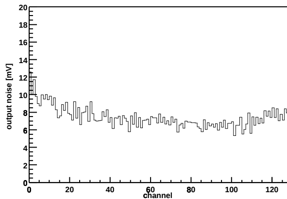
Chip Z36459A-W04-X11-Y15 Output noise vs. channel
