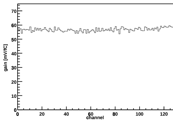
Chip Z36459A-W04-X11-Y15 Gain vs. channel
