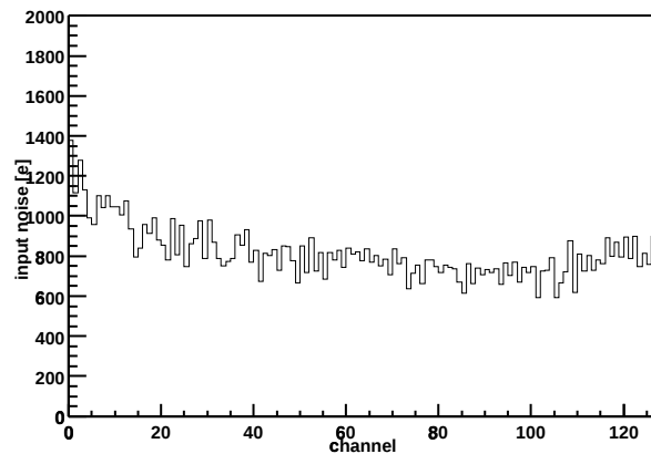
Chip Z36459A-W04-X11-Y15 Input noise vs. channel
