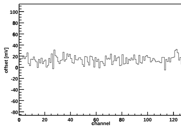
Chip Z36459A-W04-X11-Y15 Offset vs. channel
