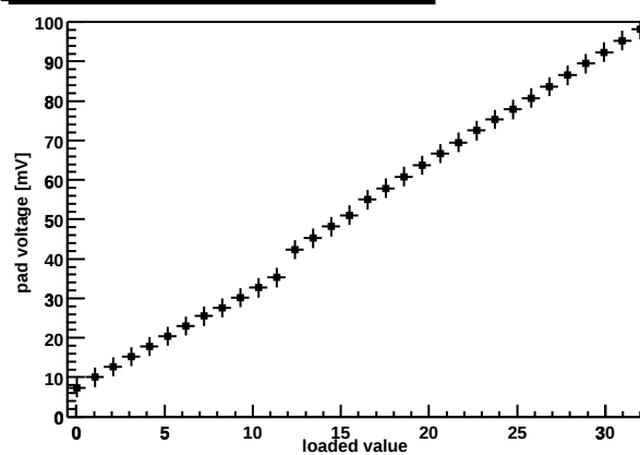
Chip Z36459A-W04-X11-Y15 preamp DAC
