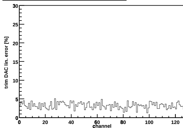
Chip Z36459A-W04-X11-Y15 trim DAC lin. error
