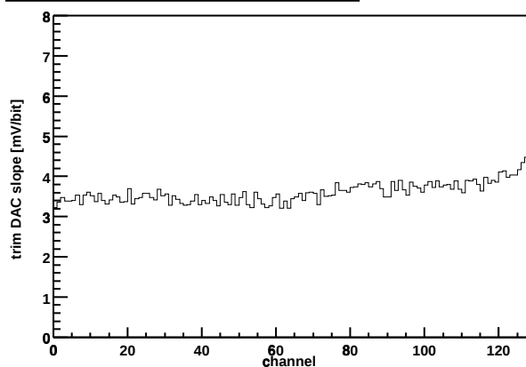
Chip Z36459A-W04-X11-Y15 Trim DAC slope vs. channel
