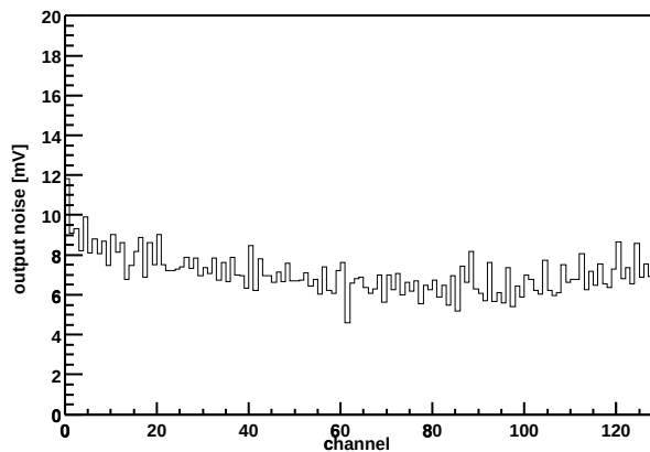
Chip Z36459A-W04-X11-Y16 Output noise vs. channel
