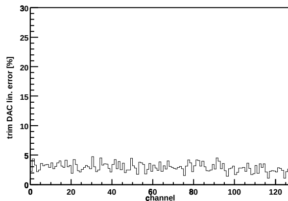
Chip Z36459A-W04-X11-Y16 trim DAC lin. error
