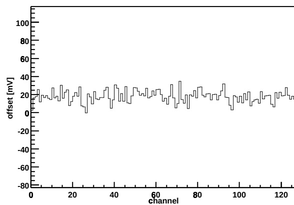
Chip Z36459A-W04-X11-Y16 Offset vs. channel
