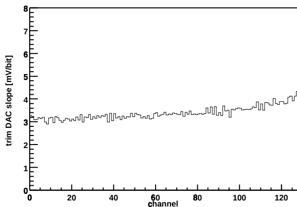
Chip Z36459A-W04-X11-Y16 Trim DAC slope vs. channel
