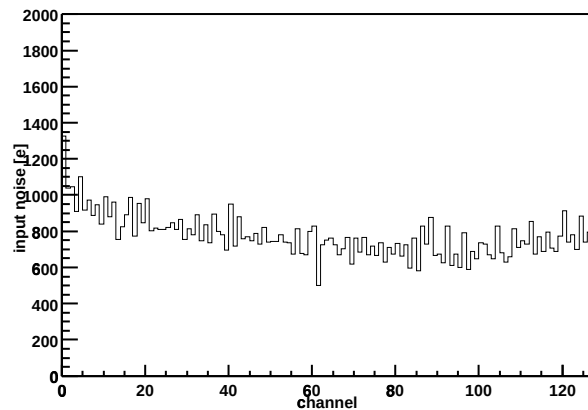
Chip Z36459A-W04-X11-Y16 Input noise vs. channel
