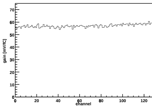
Chip Z36459A-W04-X11-Y16 Gain vs. channel
