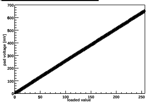
Chip Z36459A-W04-X11-Y16 threshold DAC
