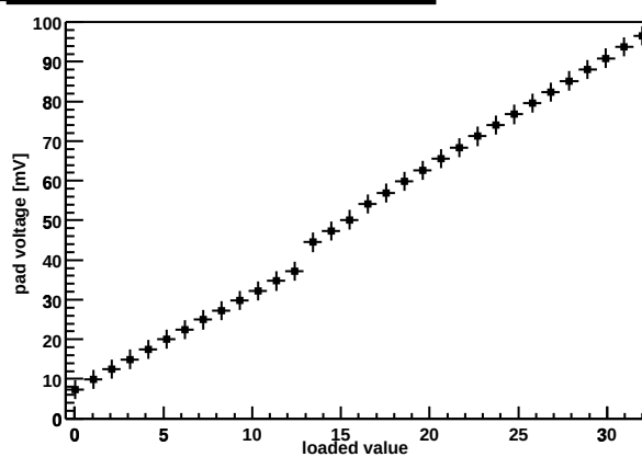
Chip Z36459A-W04-X11-Y16 preamp DAC
