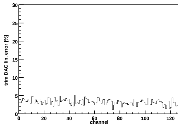
Chip Z36459A-W04-X11-Y19 trim DAC lin. error
