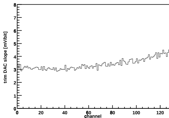
Chip Z36459A-W04-X11-Y19 Trim DAC slope vs. channel
