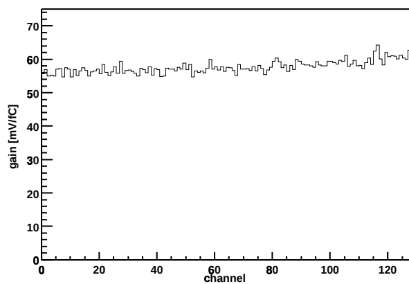
Chip Z36459A-W04-X11-Y19 Gain vs. channel
