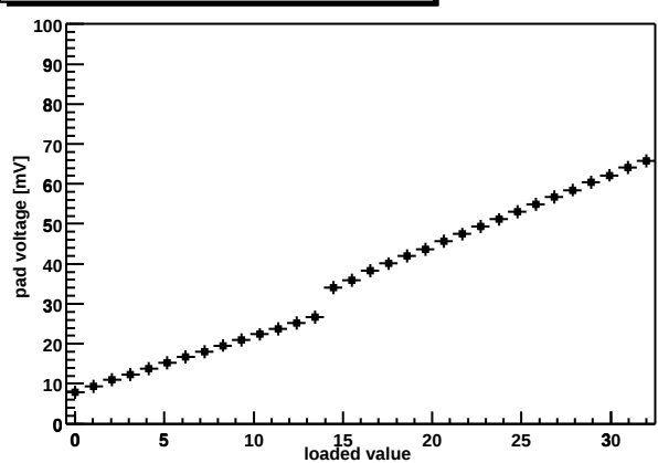
Chip Z36459A-W04-X11-Y19 shaper DAC
