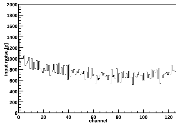
Chip Z36459A-W04-X11-Y19 Input noise vs. channel
