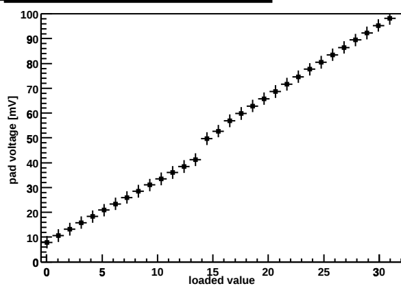
Chip Z36459A-W04-X11-Y19 preamp DAC
