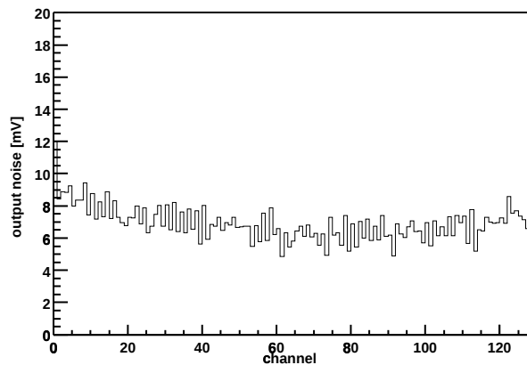
Chip Z36459A-W04-X11-Y19 Output noise vs. channel
