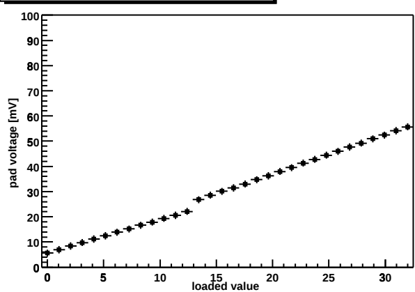
Chip Z36459A-W04-X12-Y07 shaper DAC
