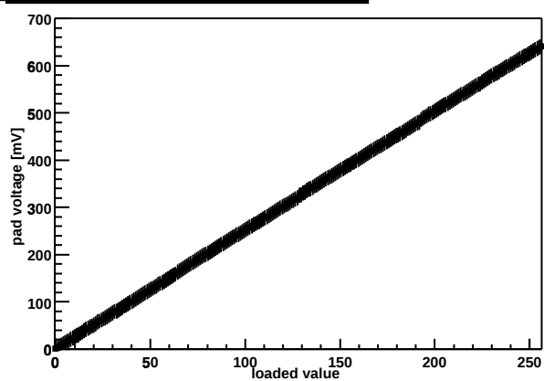
Chip Z36459A-W04-X12-Y07 threshold DAC
