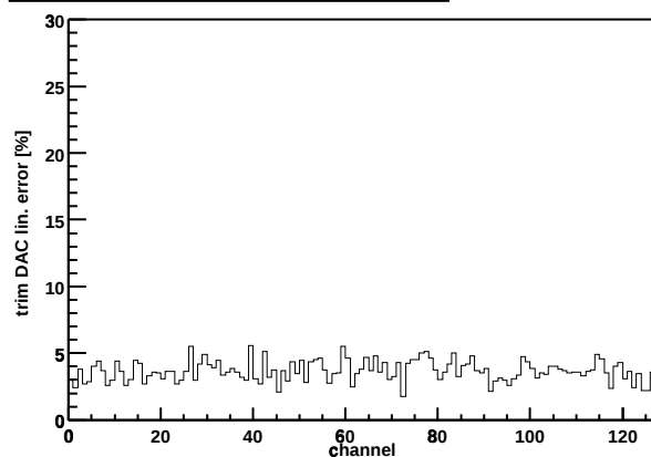
Chip Z36459A-W04-X12-Y07 trim DAC lin. error
