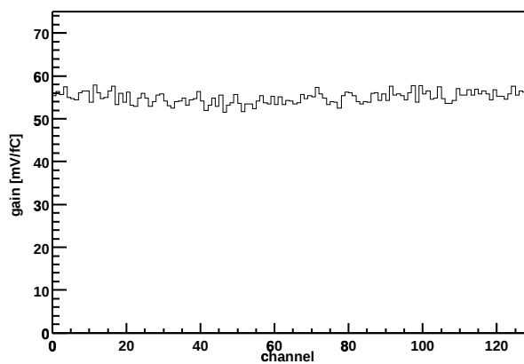
Chip Z36459A-W04-X12-Y07 Gain vs. channel
