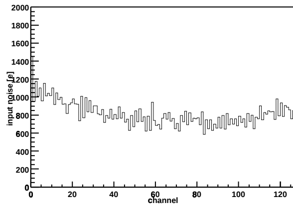
Chip Z36459A-W04-X12-Y07 Input noise vs. channel
