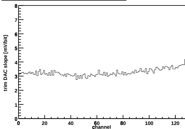
Chip Z36459A-W04-X12-Y07 Trim DAC slope vs. channel
