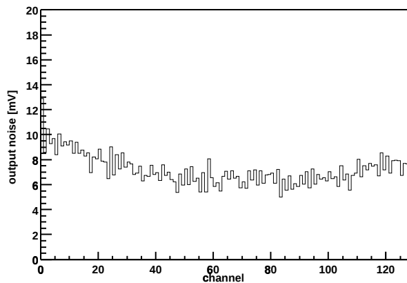
Chip Z36459A-W04-X12-Y07 Output noise vs. channel
