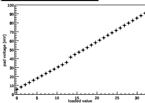
Chip Z36459A-W04-X12-Y07 preamp DAC
