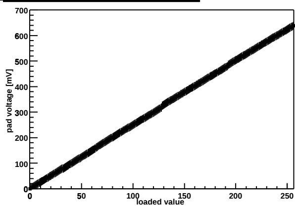
Chip Z36459A-W04-X12-Y09 threshold DAC
