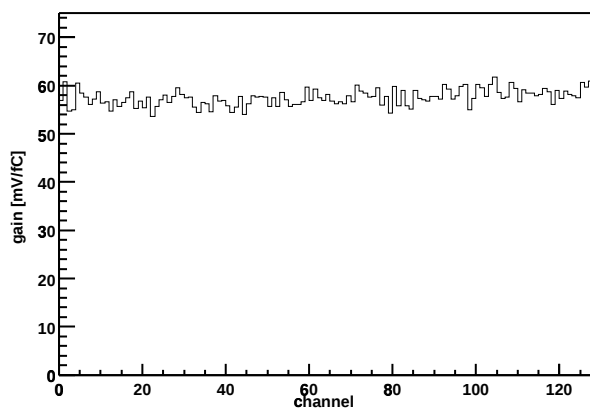
Chip Z36459A-W04-X12-Y09 Gain vs. channel
