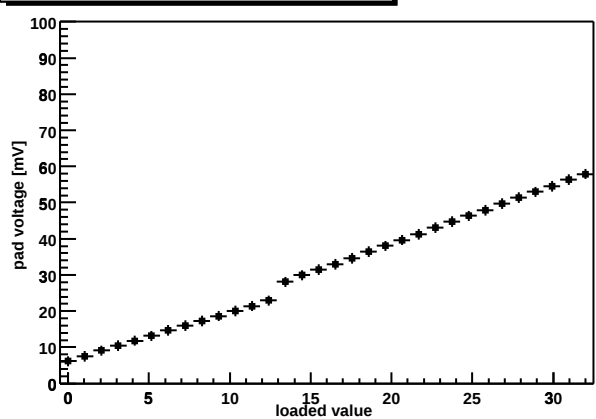
Chip Z36459A-W04-X12-Y09 shaper DAC
