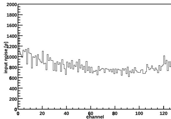
Chip Z36459A-W04-X12-Y09 Input noise vs. channel
