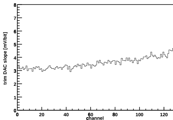
Chip Z36459A-W04-X12-Y09 Trim DAC slope vs. channel
