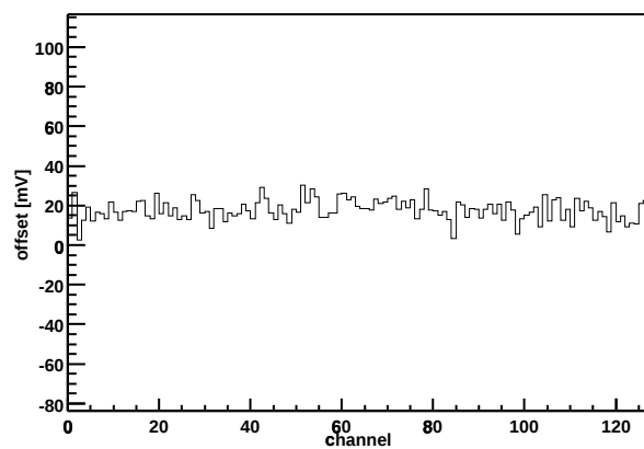
Chip Z36459A-W04-X12-Y09 Offset vs. channel
