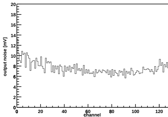
Chip Z36459A-W04-X12-Y09 Output noise vs. channel
