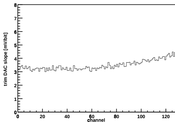
Chip Z36459A-W04-X12-Y10 Trim DAC slope vs. channel
