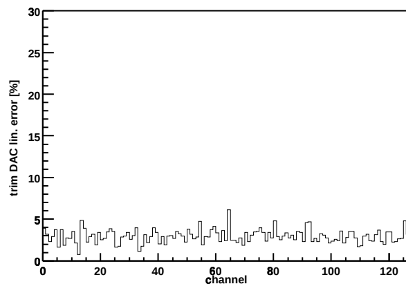
Chip Z36459A-W04-X12-Y10 trim DAC lin. error
