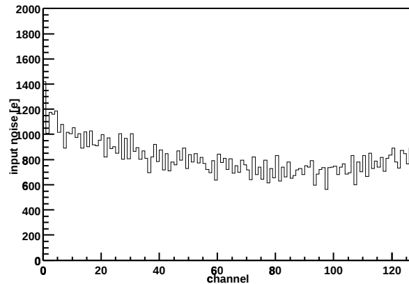
Chip Z36459A-W04-X12-Y10 Input noise vs. channel
