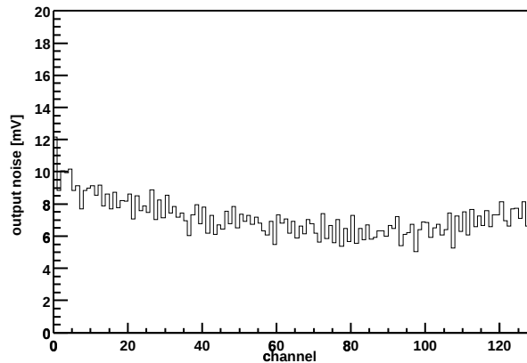
Chip Z36459A-W04-X12-Y10 Output noise vs. channel
