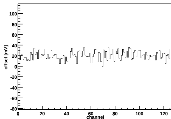
Chip Z36459A-W04-X12-Y10 Offset vs. channel
