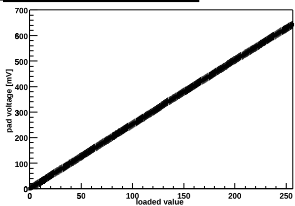
Chip Z36459A-W04-X12-Y10 threshold DAC
