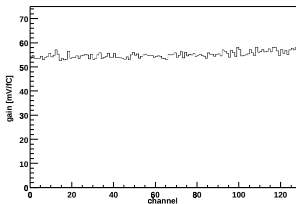
Chip Z36459A-W04-X12-Y10 Gain vs. channel
