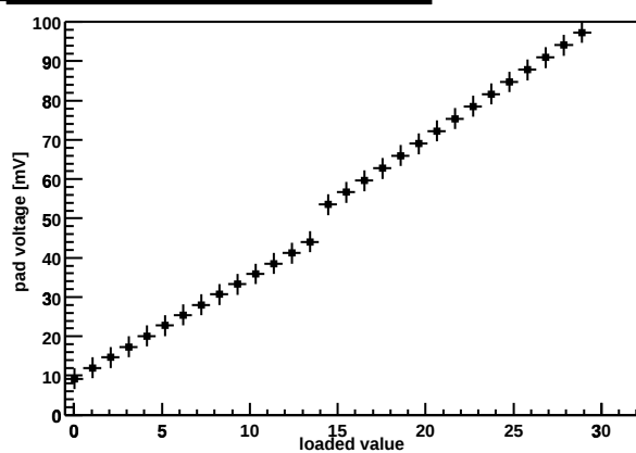
Chip Z36459A-W04-X12-Y10 preamp DAC
