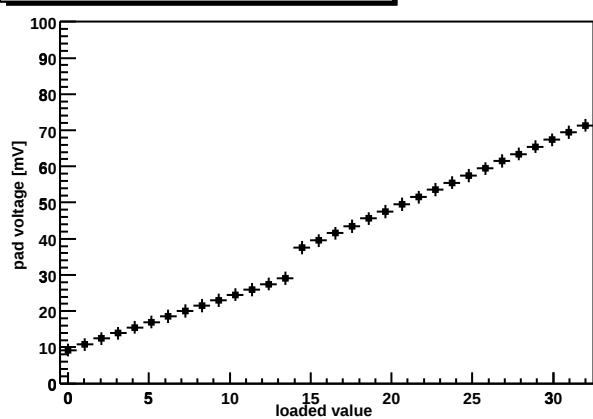
Chip Z36459A-W04-X12-Y10 shaper DAC
