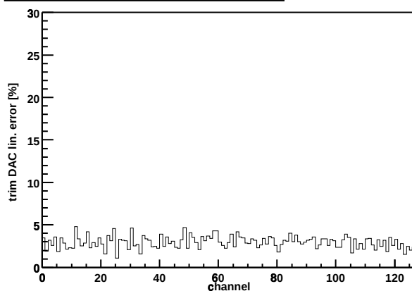
Chip Z36459A-W04-X12-Y15 trim DAC lin. error
