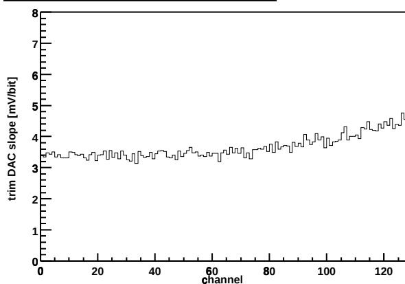
Chip Z36459A-W04-X12-Y15 Trim DAC slope vs. channel
