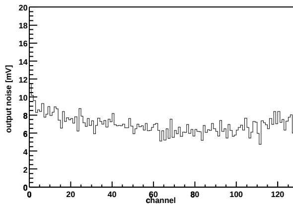
Chip Z36459A-W04-X12-Y15 Output noise vs. channel
