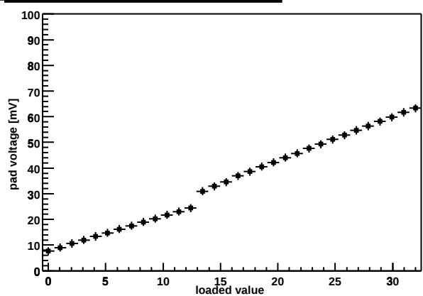
Chip Z36459A-W04-X12-Y15 shaper DAC
