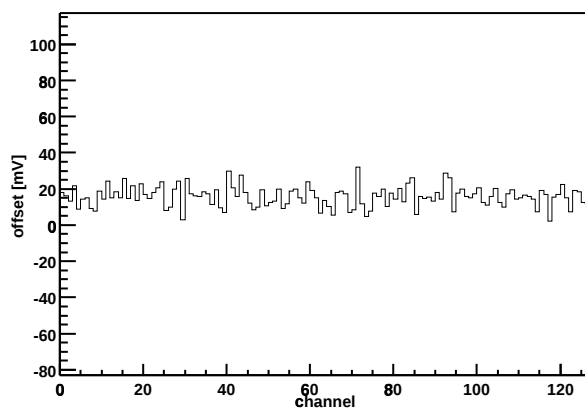
Chip Z36459A-W04-X12-Y15 Offset vs. channel
