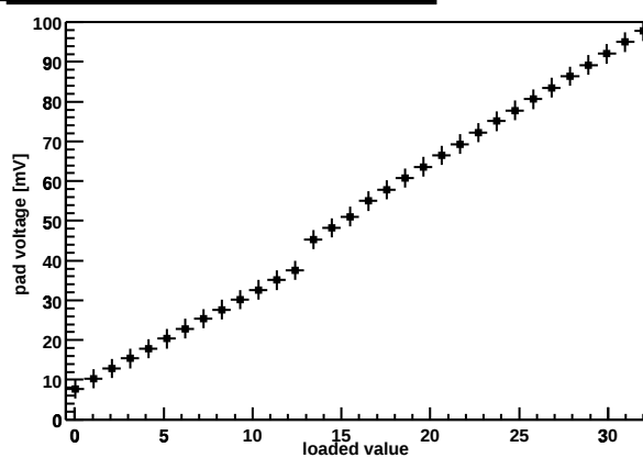
Chip Z36459A-W04-X12-Y15 preamp DAC
