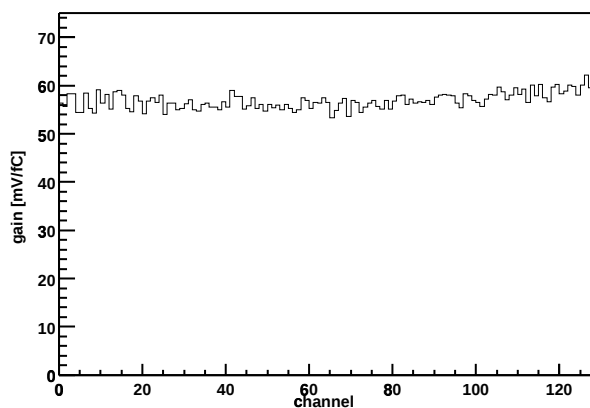
Chip Z36459A-W04-X12-Y15 Gain vs. channel
