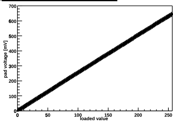
Chip Z36459A-W04-X12-Y15 threshold DAC
