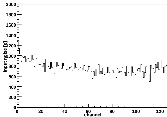
Chip Z36459A-W04-X12-Y15 Input noise vs. channel
