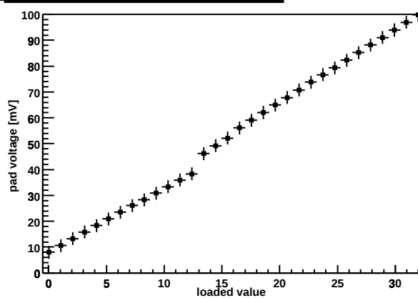
Chip Z36459A-W04-X12-Y16 preamp DAC
