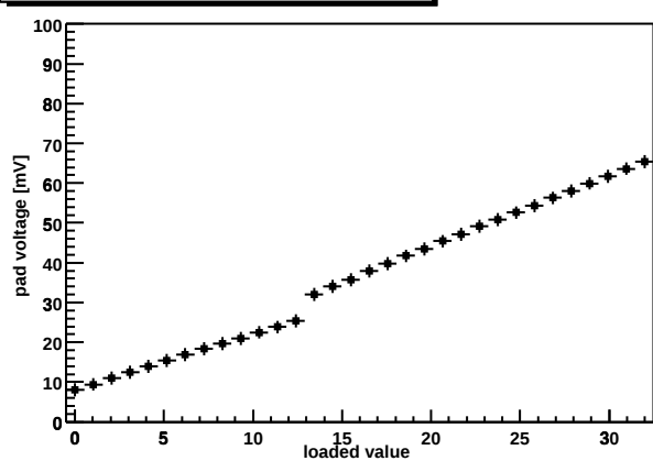
Chip Z36459A-W04-X12-Y16 shaper DAC
