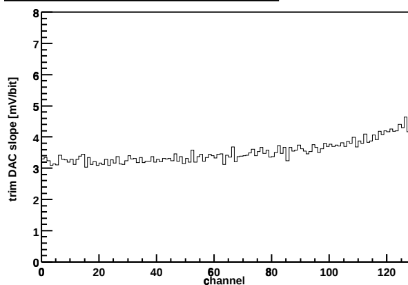
Chip Z36459A-W04-X12-Y16 Trim DAC slope vs. channel
