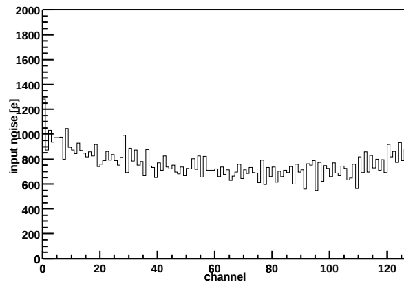
Chip Z36459A-W04-X12-Y16 Input noise vs. channel
