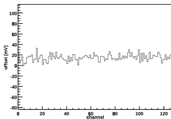
Chip Z36459A-W04-X12-Y16 Offset vs. channel
