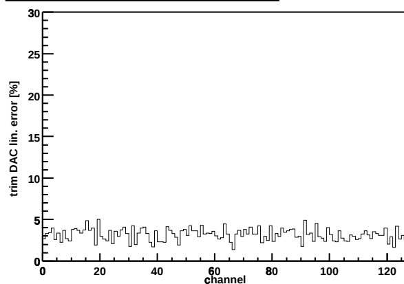
Chip Z36459A-W04-X12-Y16 trim DAC lin. error
