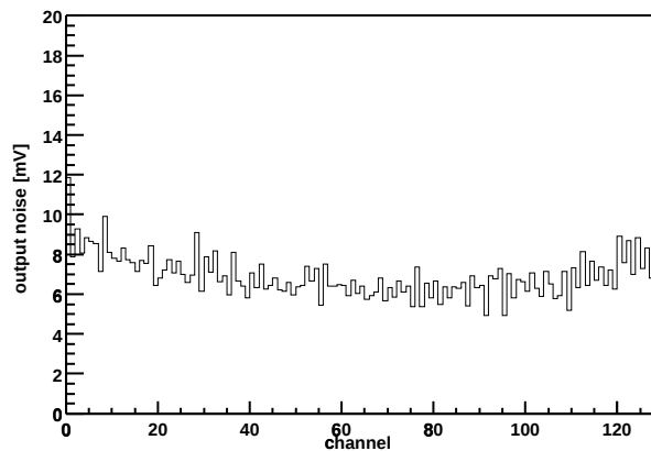
Chip Z36459A-W04-X12-Y16 Output noise vs. channel
