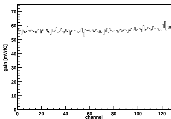
Chip Z36459A-W04-X12-Y16 Gain vs. channel
