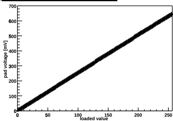
Chip Z36459A-W04-X13-Y07 threshold DAC
