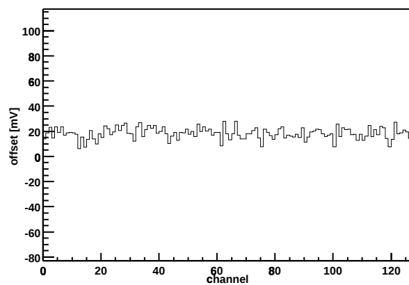
Chip Z36459A-W04-X13-Y07 Offset vs. channel
