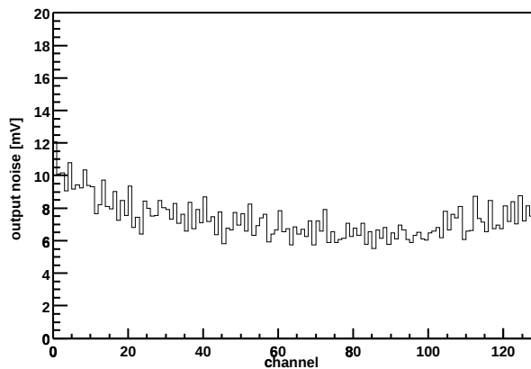
Chip Z36459A-W04-X13-Y07 Output noise vs. channel
