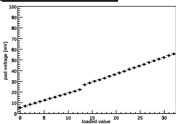
Chip Z36459A-W04-X13-Y07 shaper DAC
