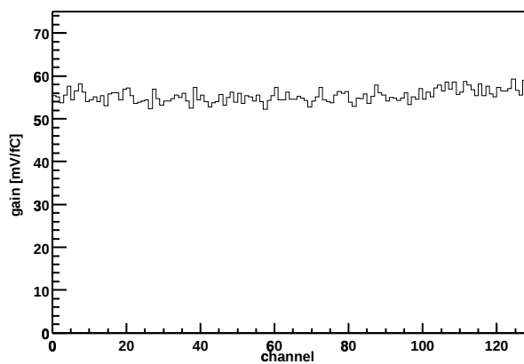
Chip Z36459A-W04-X13-Y07 Gain vs. channel
