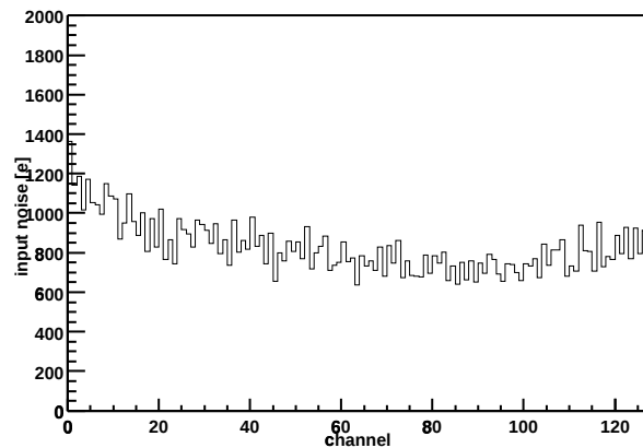
Chip Z36459A-W04-X13-Y07 Input noise vs. channel
