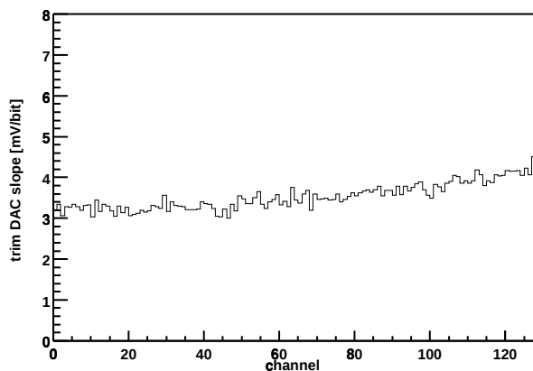
Chip Z36459A-W04-X13-Y07 Trim DAC slope vs. channel
