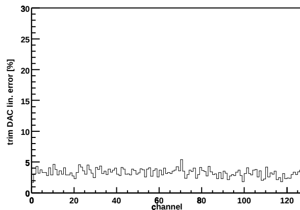
Chip Z36459A-W04-X13-Y07 trim DAC lin. error
