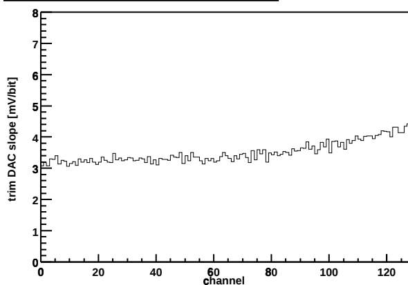
Chip Z36459A-W04-X13-Y08 Trim DAC slope vs. channel
