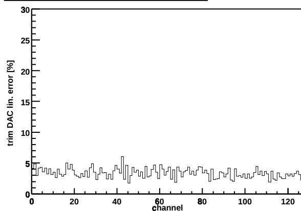
Chip Z36459A-W04-X13-Y08 trim DAC lin. error
