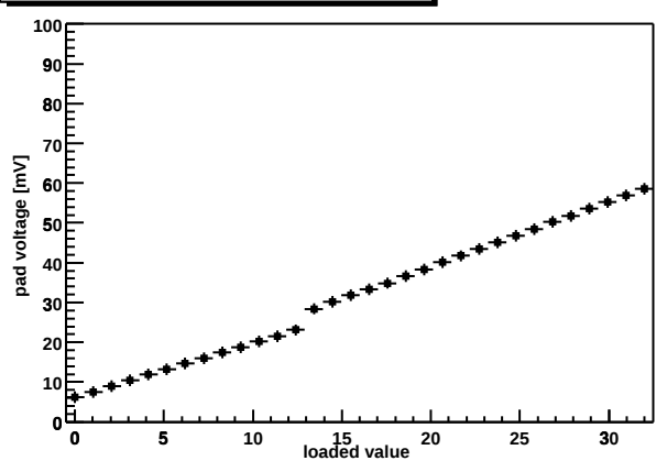
Chip Z36459A-W04-X13-Y08 shaper DAC
