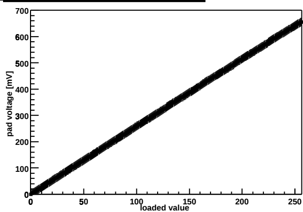
Chip Z36459A-W04-X13-Y08 threshold DAC
