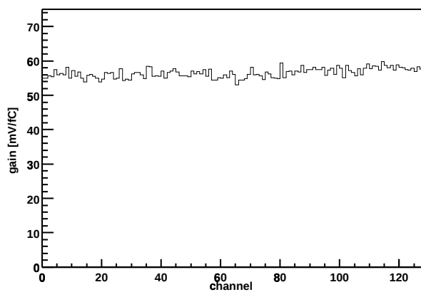
Chip Z36459A-W04-X13-Y08 Gain vs. channel
