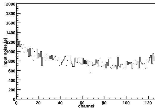
Chip Z36459A-W04-X13-Y08 Input noise vs. channel
