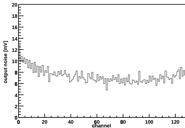
Chip Z36459A-W04-X13-Y08 Output noise vs. channel
