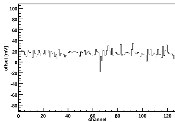
Chip Z36459A-W04-X13-Y08 Offset vs. channel
