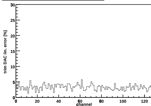
Chip Z36459A-W04-X13-Y10 trim DAC lin. error
