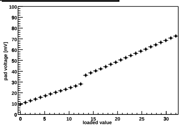
Chip Z36459A-W04-X13-Y10 shaper DAC
