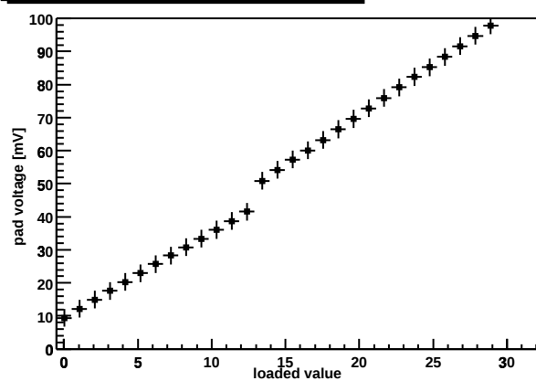
Chip Z36459A-W04-X13-Y10 preamp DAC
