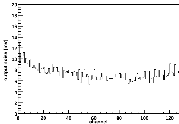
Chip Z36459A-W04-X13-Y10 Output noise vs. channel
