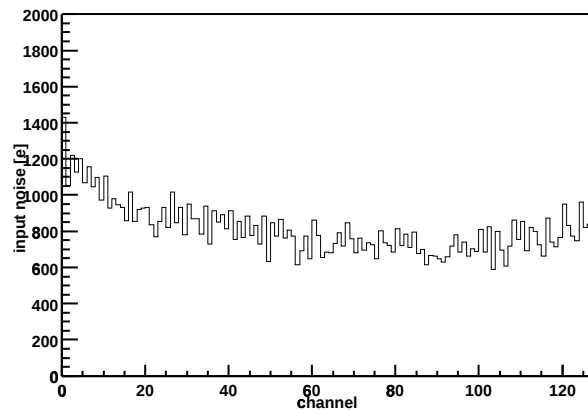
Chip Z36459A-W04-X13-Y10 Input noise vs. channel
