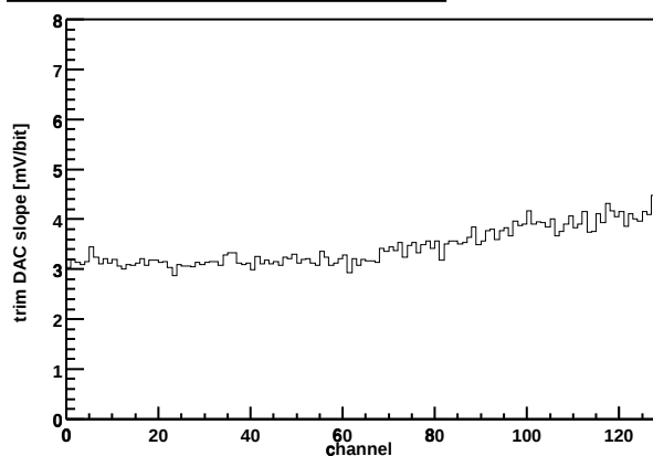
Chip Z36459A-W04-X13-Y10 Trim DAC slope vs. channel
