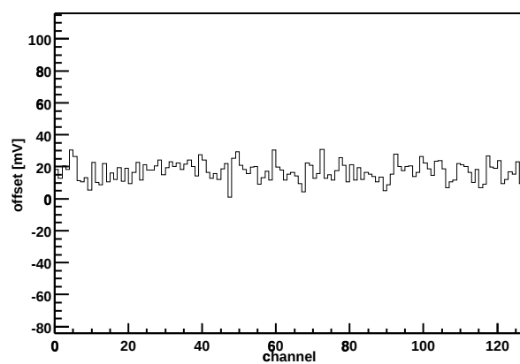
Chip Z36459A-W04-X13-Y10 Offset vs. channel
