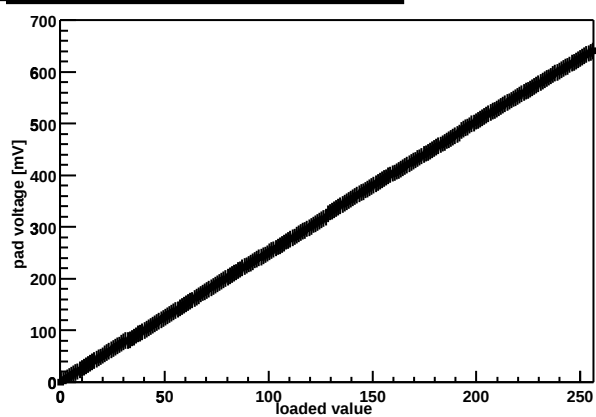
Chip Z36459A-W04-X13-Y10 threshold DAC
