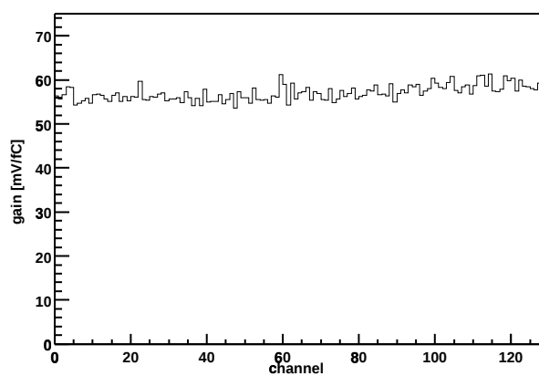
Chip Z36459A-W04-X13-Y10 Gain vs. channel
