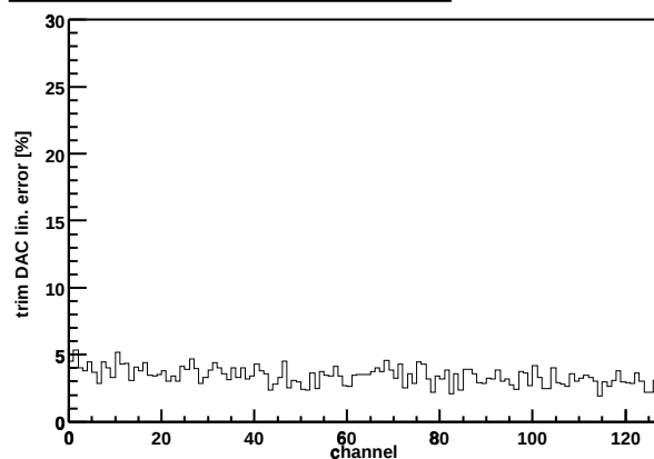
Chip Z36459A-W04-X13-Y17 trim DAC lin. error
