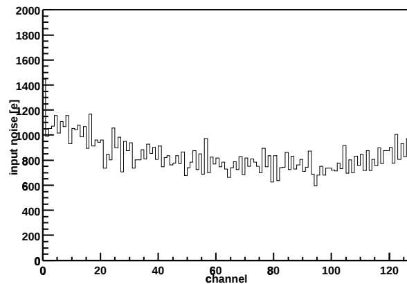
Chip Z36459A-W04-X13-Y17 Input noise vs. channel
