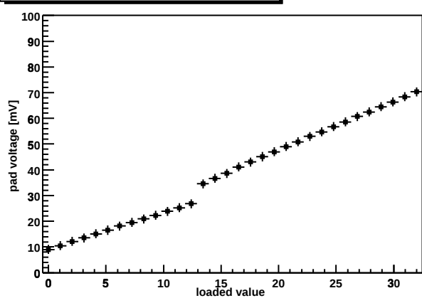
Chip Z36459A-W04-X13-Y17 shaper DAC
