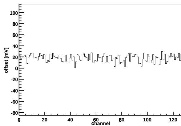
Chip Z36459A-W04-X13-Y17 Offset vs. channel
