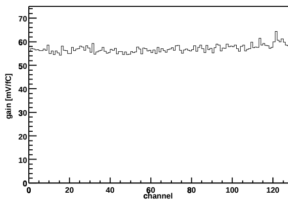
Chip Z36459A-W04-X13-Y17 Gain vs. channel
