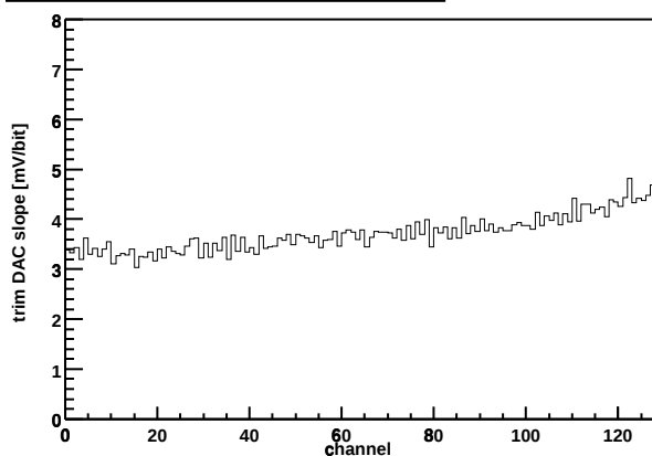
Chip Z36459A-W04-X13-Y17 Trim DAC slope vs. channel
