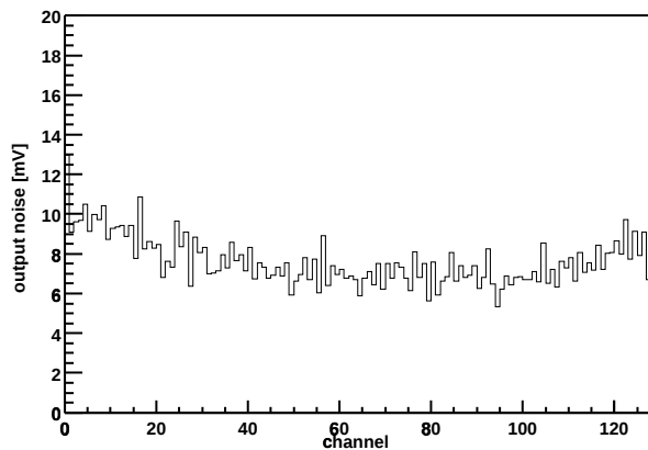
Chip Z36459A-W04-X13-Y17 Output noise vs. channel
