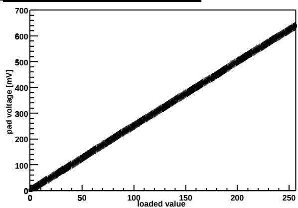
Chip Z36459A-W04-X13-Y17 threshold DAC
