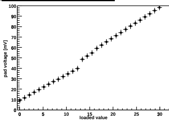
Chip Z36459A-W04-X13-Y17 preamp DAC
