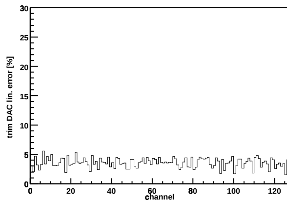
Chip Z36459A-W04-X14-Y12 trim DAC lin. error
