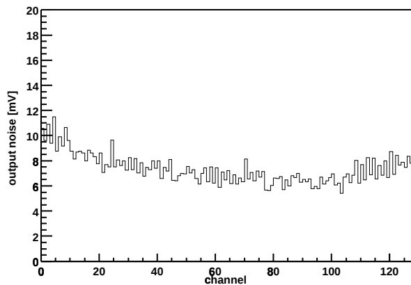
Chip Z36459A-W04-X14-Y12 Output noise vs. channel
