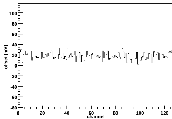
Chip Z36459A-W04-X14-Y12 Offset vs. channel
