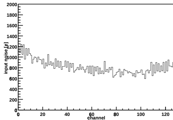
Chip Z36459A-W04-X14-Y12 Input noise vs. channel
