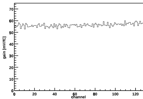
Chip Z36459A-W04-X14-Y12 Gain vs. channel
