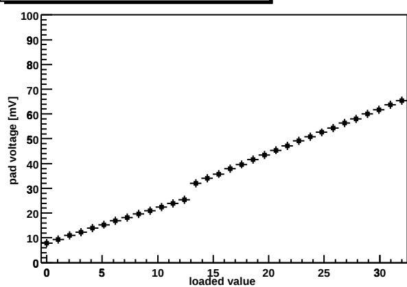
Chip Z36459A-W04-X14-Y12 shaper DAC
