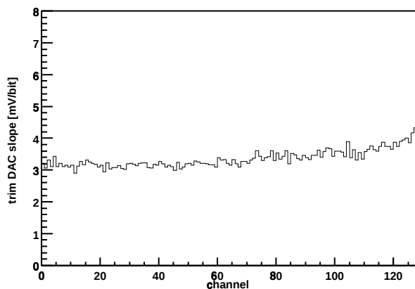
Chip Z36459A-W04-X14-Y12 Trim DAC slope vs. channel
