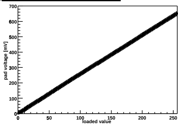
Chip Z36459A-W04-X14-Y12 threshold DAC
