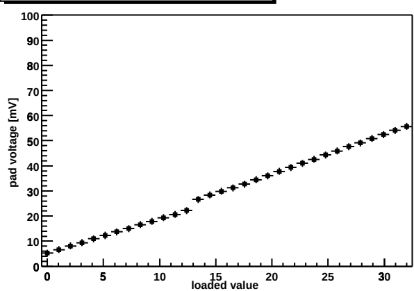
Chip Z36459A-W04-X15-Y05 shaper DAC
