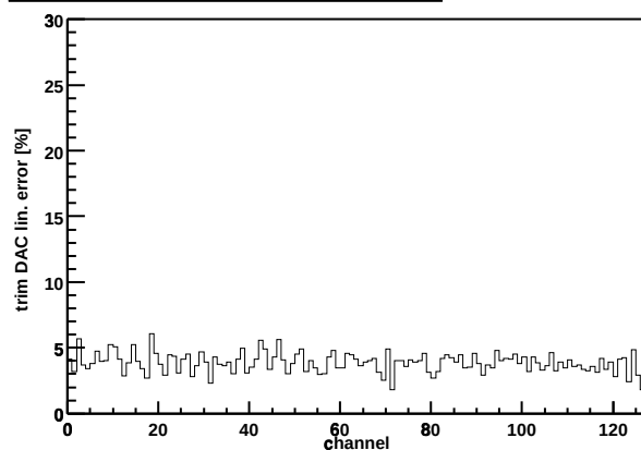
Chip Z36459A-W04-X15-Y05 trim DAC lin. error
