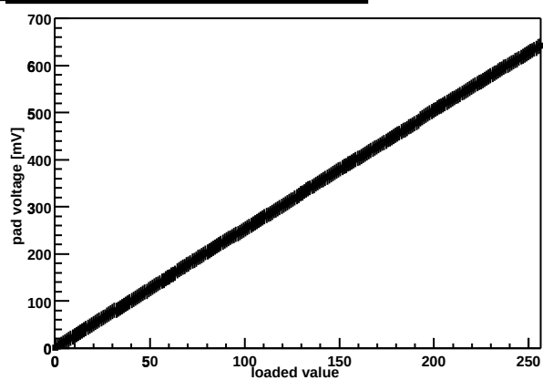
Chip Z36459A-W04-X15-Y05 threshold DAC
