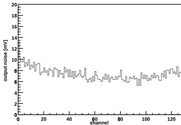
Chip Z36459A-W04-X15-Y05 Output noise vs. channel
