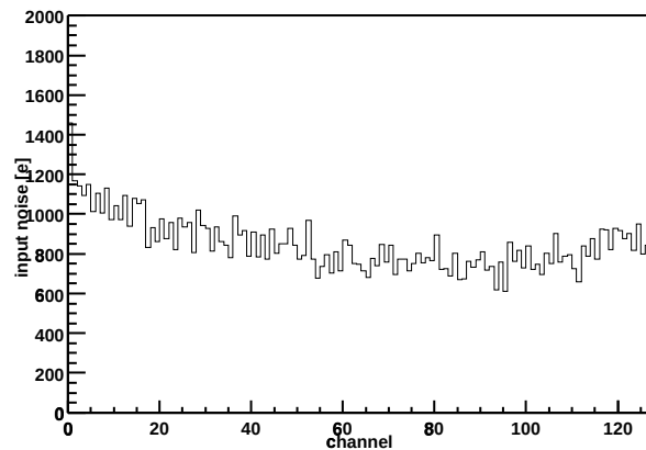
Chip Z36459A-W04-X15-Y05 Input noise vs. channel
