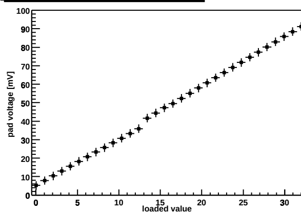
Chip Z36459A-W04-X15-Y05 preamp DAC
