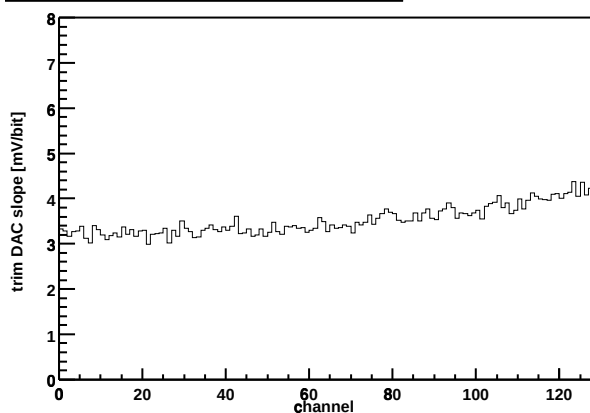
Chip Z36459A-W04-X15-Y05 Trim DAC slope vs. channel
