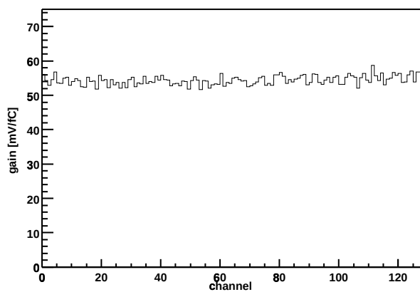
Chip Z36459A-W04-X15-Y05 Gain vs. channel
