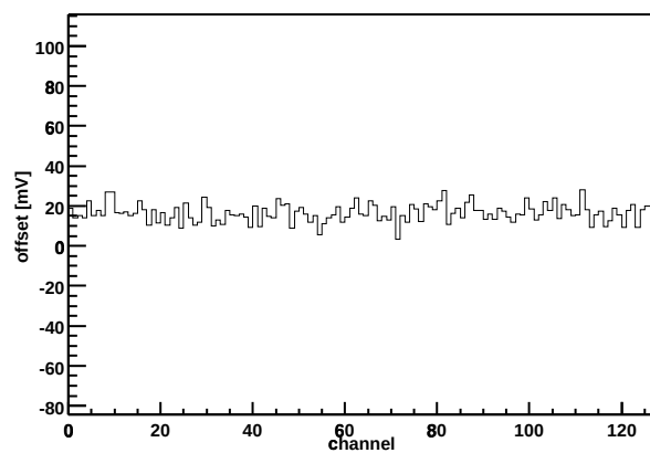
Chip Z36459A-W04-X15-Y05 Offset vs. channel
