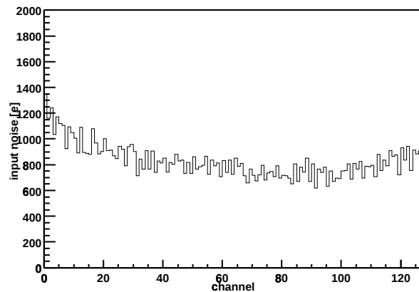
Chip Z36459A-W04-X15-Y10 Input noise vs. channel
