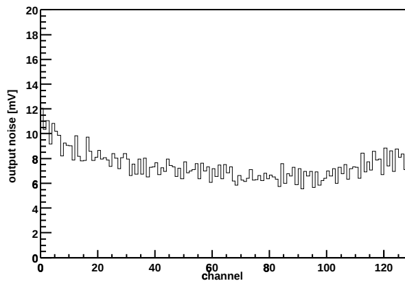
Chip Z36459A-W04-X15-Y10 Output noise vs. channel
