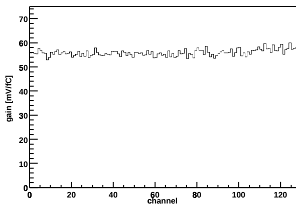
Chip Z36459A-W04-X15-Y10 Gain vs. channel
