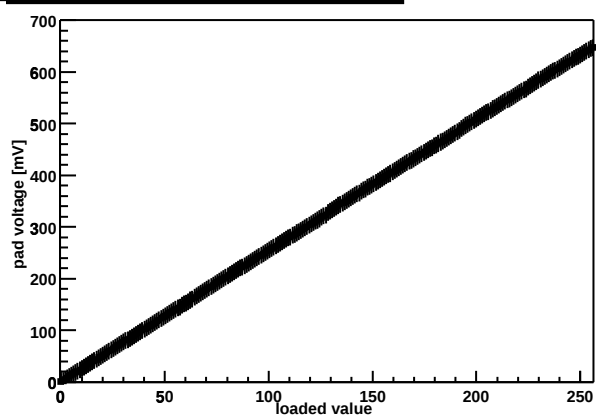
Chip Z36459A-W04-X15-Y10 threshold DAC
