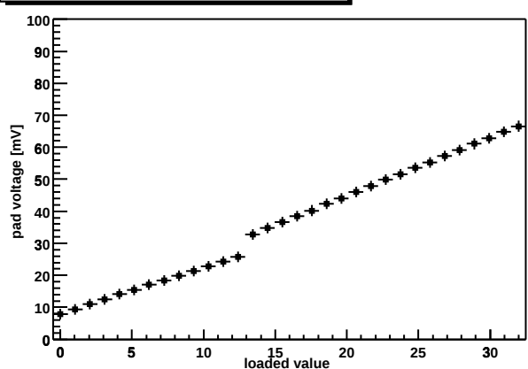
Chip Z36459A-W04-X15-Y10 shaper DAC
