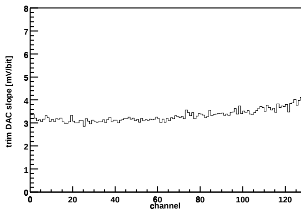
Chip Z36459A-W04-X15-Y10 Trim DAC slope vs. channel
