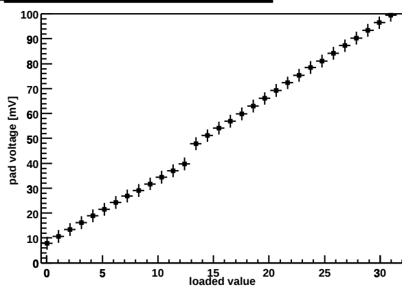
Chip Z36459A-W04-X15-Y10 preamp DAC
