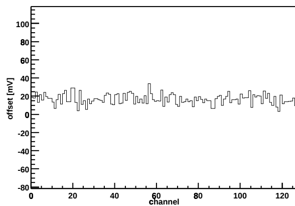
Chip Z36459A-W04-X15-Y10 Offset vs. channel
