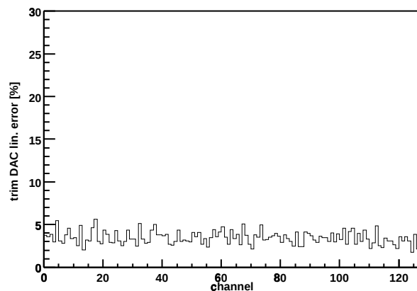
Chip Z36459A-W04-X15-Y10 trim DAC lin. error
