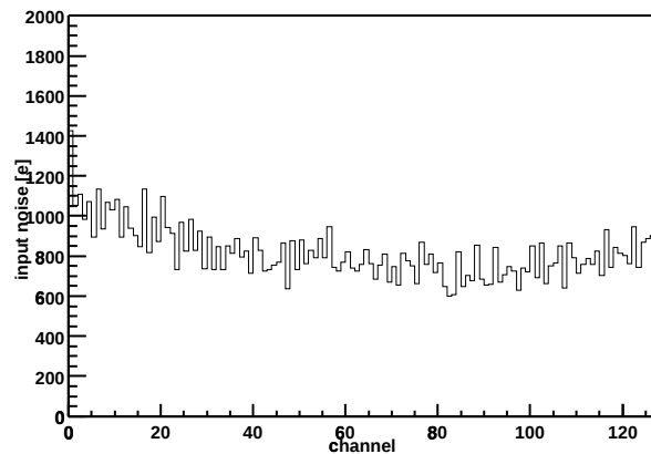
Chip Z36459A-W04-X15-Y11 Input noise vs. channel
