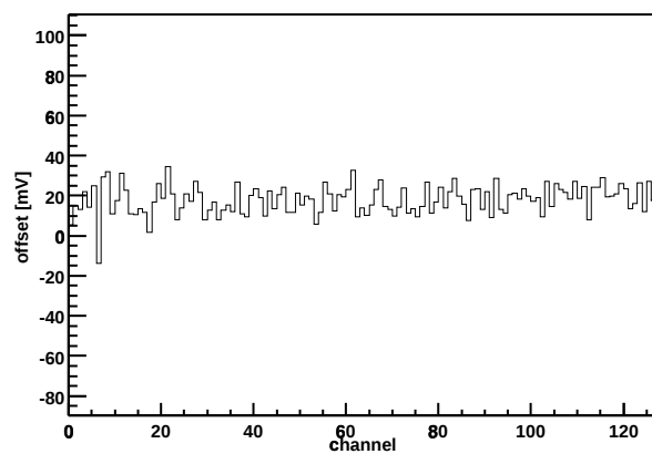
Chip Z36459A-W04-X15-Y11 Offset vs. channel
