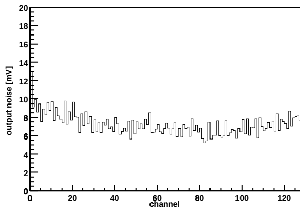
Chip Z36459A-W04-X15-Y11 Output noise vs. channel
