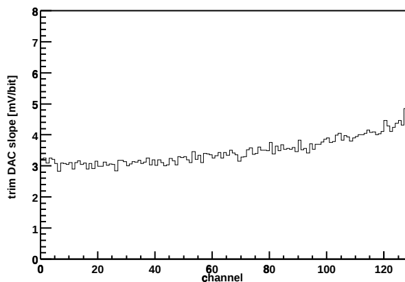
Chip Z36459A-W04-X15-Y11 Trim DAC slope vs. channel
