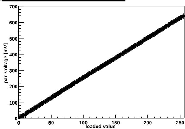
Chip Z36459A-W04-X15-Y11 threshold DAC
