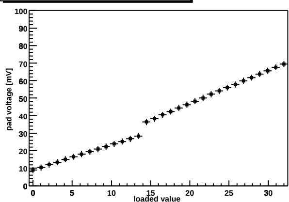
Chip Z36459A-W04-X15-Y11 shaper DAC
