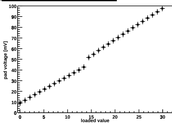
Chip Z36459A-W04-X15-Y11 preamp DAC
