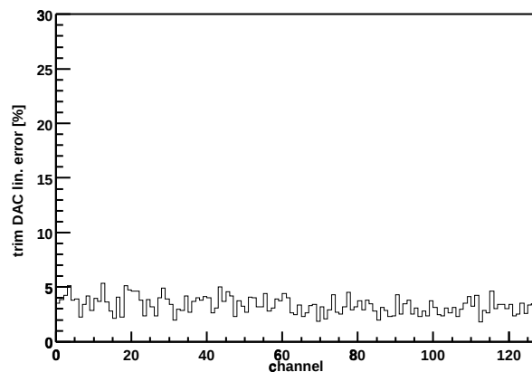
Chip Z36459A-W04-X15-Y11 trim DAC lin. error
