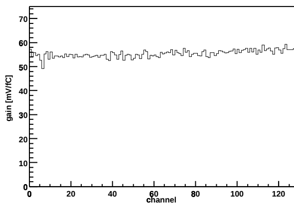
Chip Z36459A-W04-X15-Y11 Gain vs. channel
