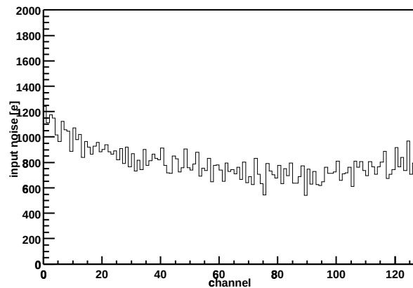
Chip Z36459A-W04-X15-Y12 Input noise vs. channel
