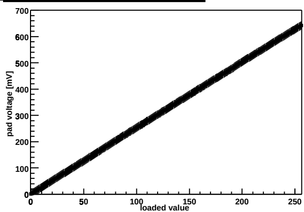
Chip Z36459A-W04-X15-Y12 threshold DAC
