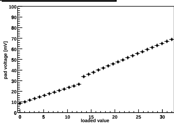
Chip Z36459A-W04-X15-Y12 shaper DAC
