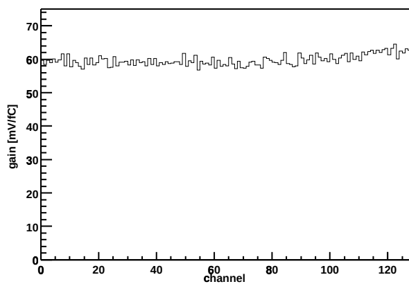
Chip Z36459A-W04-X15-Y12 Gain vs. channel
