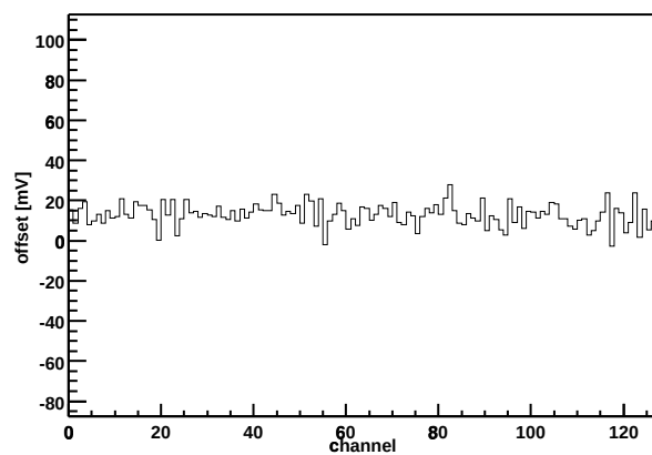
Chip Z36459A-W04-X15-Y12 Offset vs. channel
