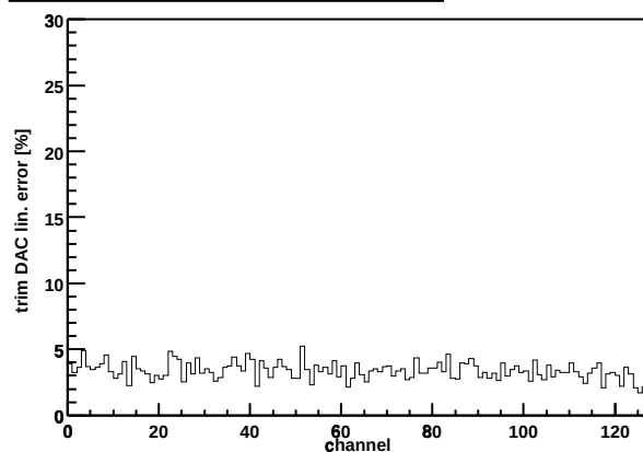
Chip Z36459A-W04-X15-Y12 trim DAC lin. error
