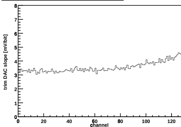
Chip Z36459A-W04-X15-Y12 Trim DAC slope vs. channel
