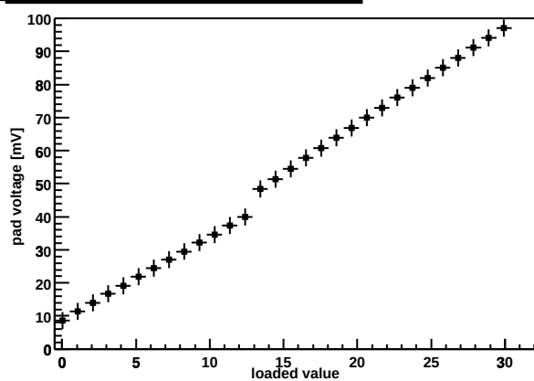
Chip Z36459A-W04-X15-Y12 preamp DAC
