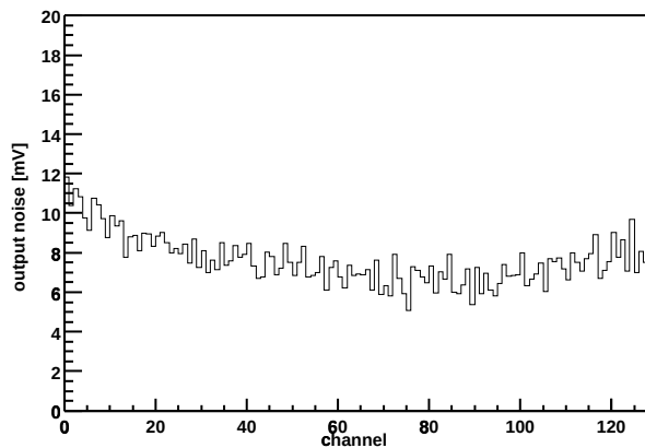
Chip Z36459A-W04-X15-Y12 Output noise vs. channel
